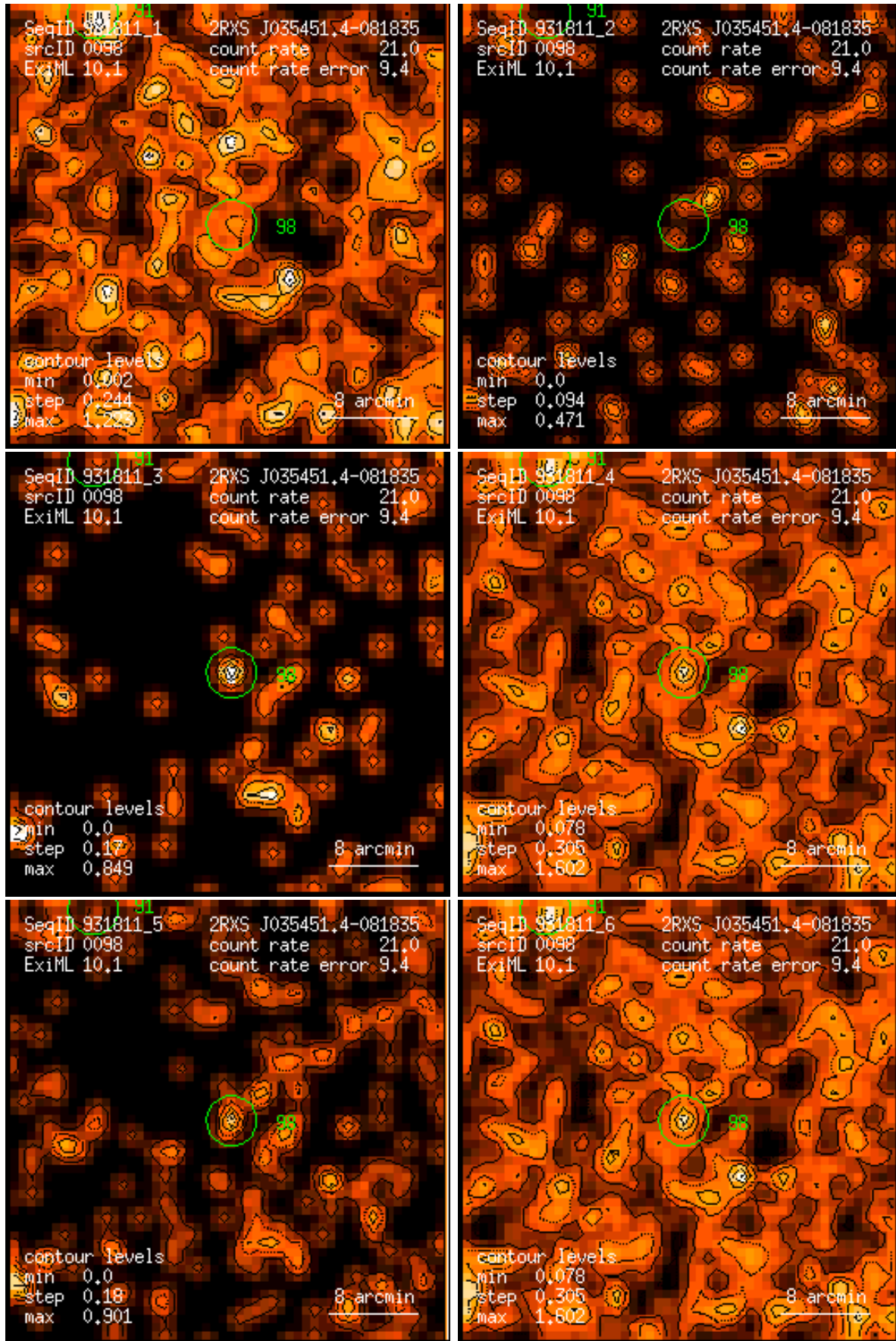
Figure 98: RASS 931811: detection 0098: band rate images, Gaussian filter: (1) PSPC channels 11 – 41, (2) 52 – 90, (3) 91 – 201, (4) 11 – 235, (5) 52 – 201, (6) 11 – 201. Broad band rates in counts/ks. Band rate contour levels in counts/ks/arcmin 2 .
