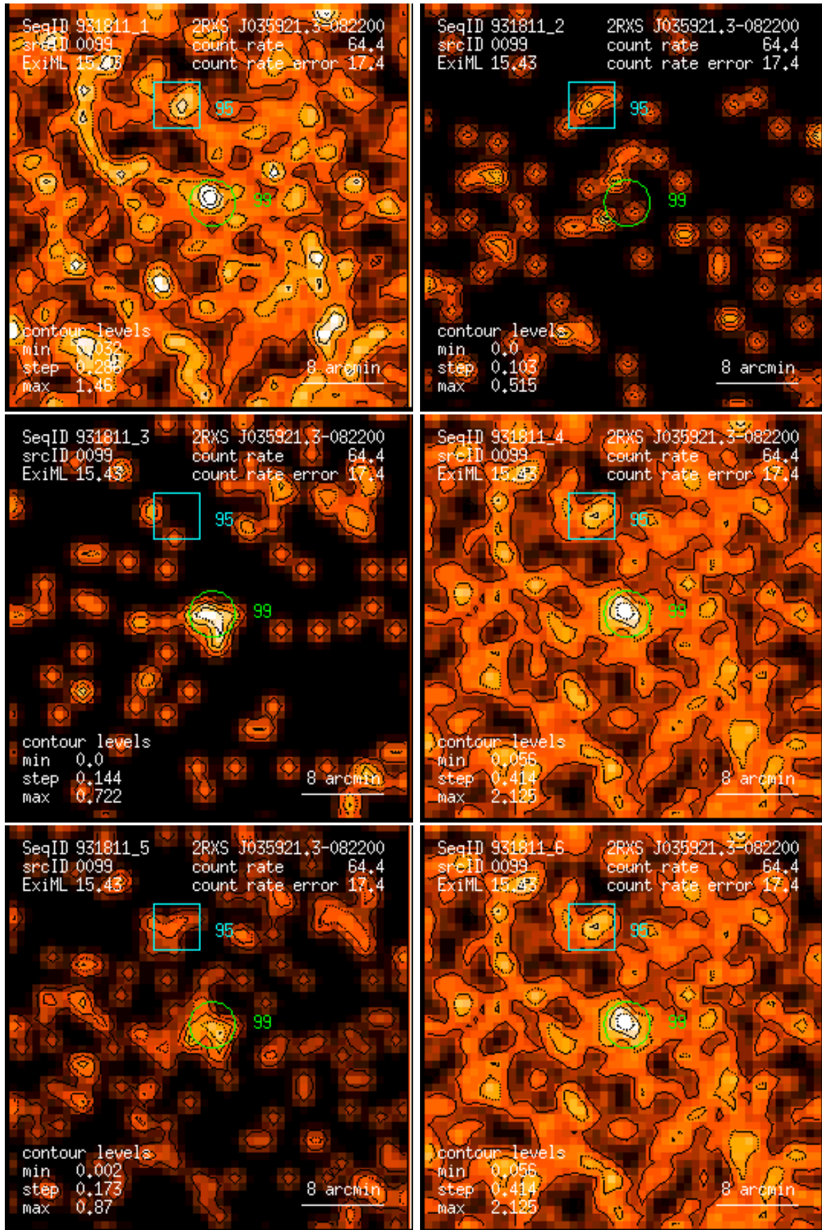
Figure 99: RASS 931811: detection 0099: band rate images, Gaussian filter: (1) PSPC channels 11 – 41, (2) 52 – 90, (3) 91 – 201, (4) 11 – 235, (5) 52 – 201, (6) 11 – 201. Broad band rates in counts/ks. Band rate contour levels in counts/ks/arcmin 2 .
