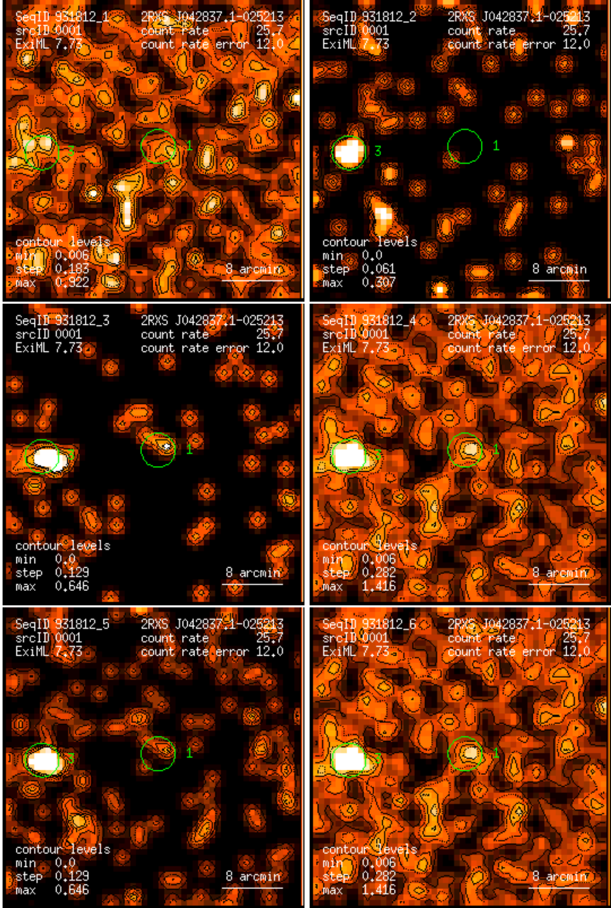
Figure 1: RASS 931812: detection 0001: band rate images, Gaussian filter: (1) PSPC channels 11 – 41, (2) 52 – 90, (3) 91 – 201, (4) 11 – 235, (5) 52 – 201, (6) 11 – 201. Broad band rates in counts/ks. Band rate contour levels in counts/ks/arcmin 2 .
