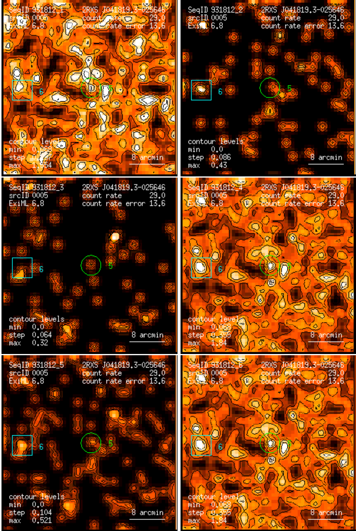
Figure 5: RASS 931812: detection 0005: band rate images, Gaussian filter: (1) PSPC channels 11 – 41, (2) 52 – 90, (3) 91 – 201, (4) 11 – 235, (5) 52 – 201, (6) 11 – 201. Broad band rates in counts/ks. Band rate contour levels in counts/ks/arcmin 2 .
