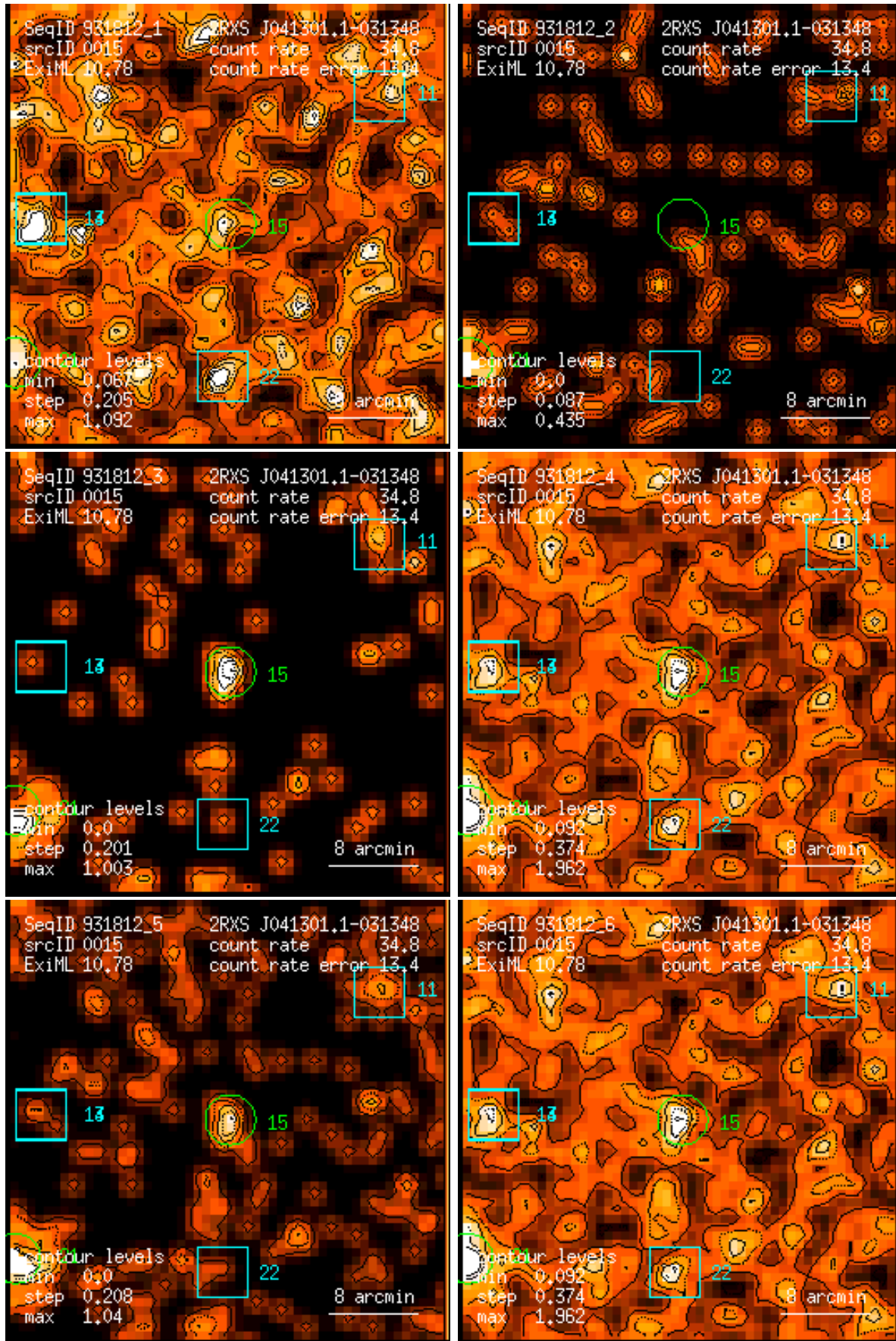
Figure 15: RASS 931812: detection 0015: band rate images, Gaussian filter: (1) PSPC channels 11 – 41, (2) 52 – 90, (3) 91 – 201, (4) 11 – 235, (5) 52 – 201, (6) 11 – 201. Broad band rates in counts/ks. Band rate contour levels in counts/ks/arcmin 2 .
