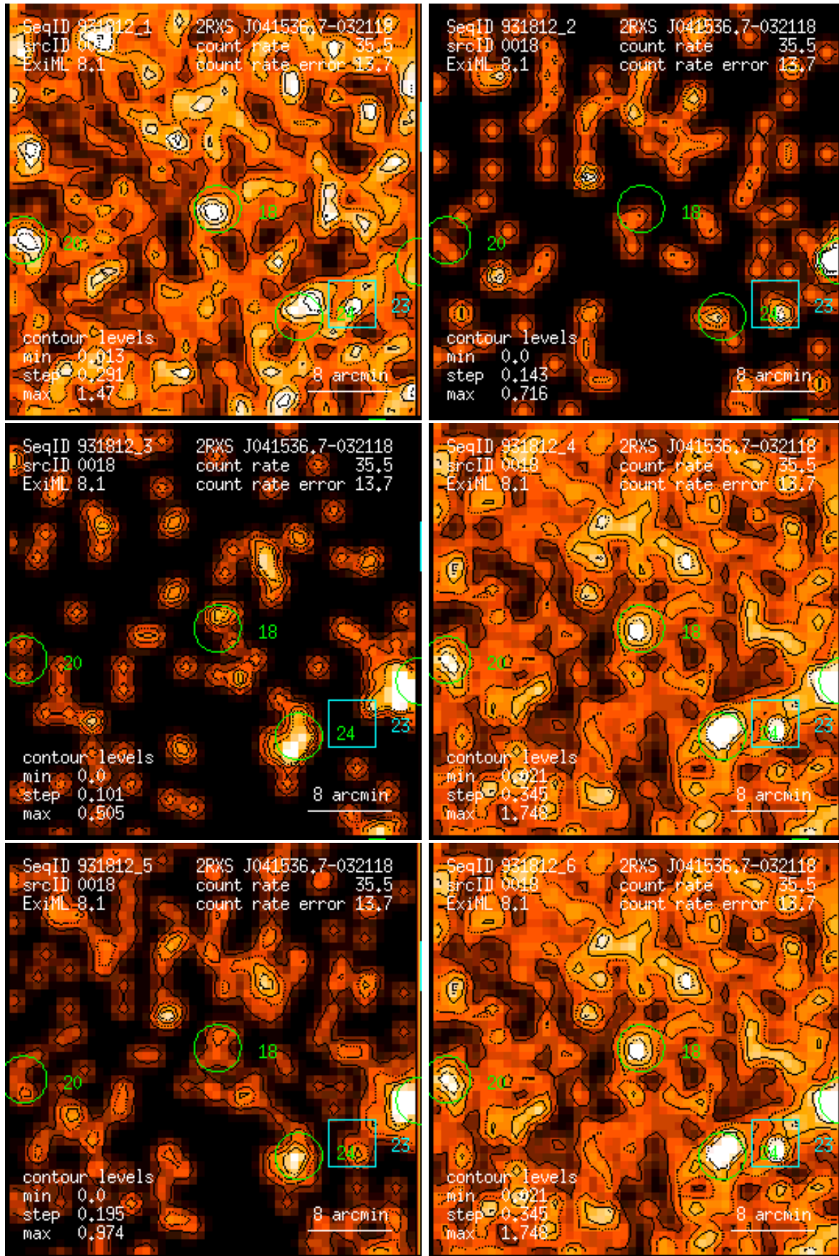
Figure 18: RASS 931812: detection 0018: band rate images, Gaussian filter: (1) PSPC channels 11 – 41, (2) 52 – 90, (3) 91 – 201, (4) 11 – 235, (5) 52 – 201, (6) 11 – 201. Broad band rates in counts/ks. Band rate contour levels in counts/ks/arcmin 2 .
