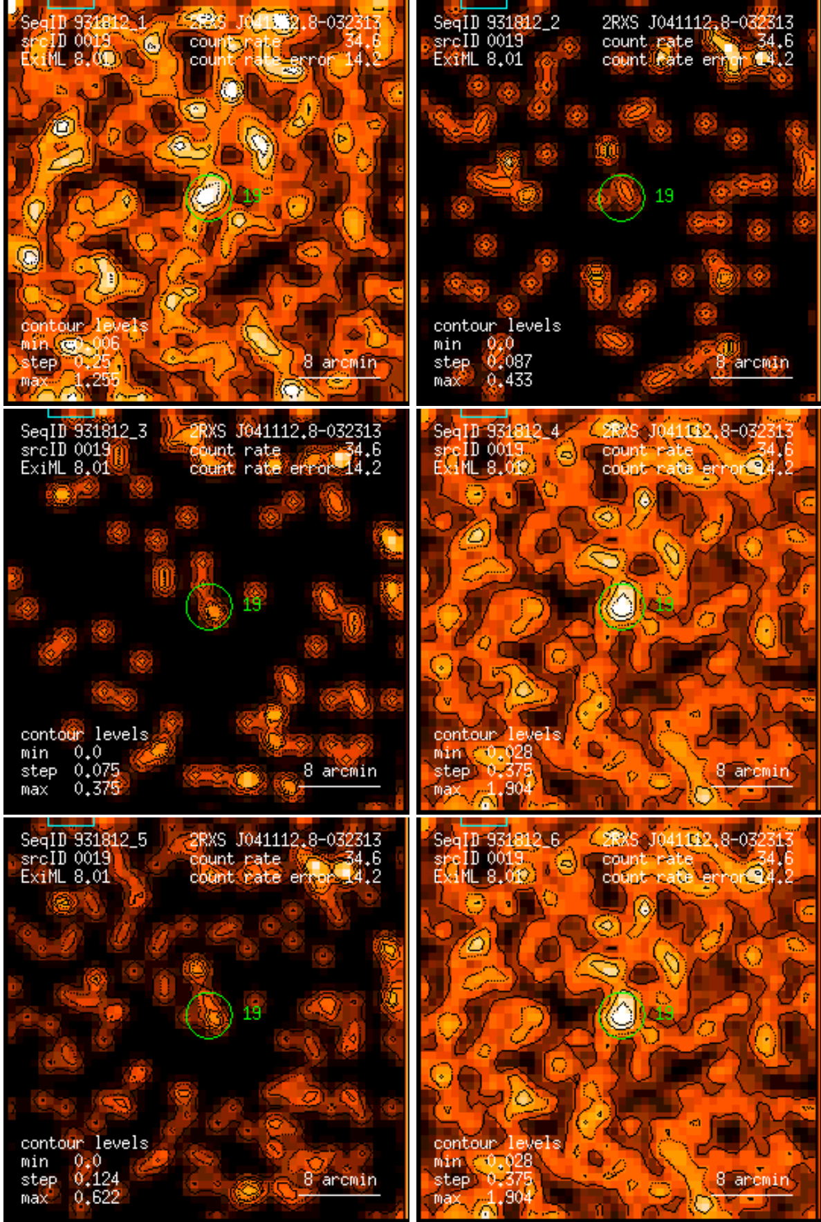
Figure 19: RASS 931812: detection 0019: band rate images, Gaussian filter: (1) PSPC channels 11 – 41, (2) 52 – 90, (3) 91 – 201, (4) 11 – 235, (5) 52 – 201, (6) 11 – 201. Broad band rates in counts/ks. Band rate contour levels in counts/ks/arcmin 2 .
