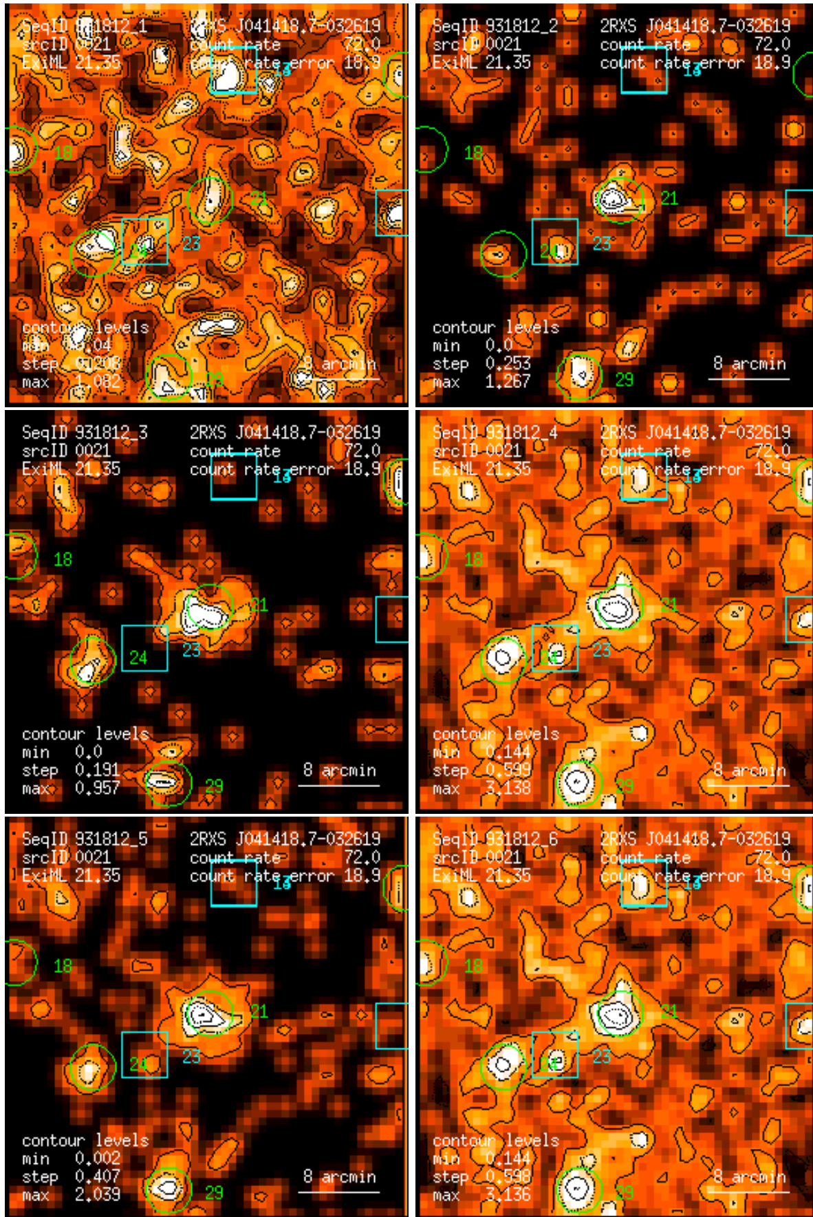
Figure 21: RASS 931812: detection 0021: band rate images, Gaussian filter: (1) PSPC channels 11 – 41, (2) 52 – 90, (3) 91 – 201, (4) 11 – 235, (5) 52 – 201, (6) 11 – 201. Broad band rates in counts/ks. Band rate contour levels in counts/ks/arcmin 2 .
