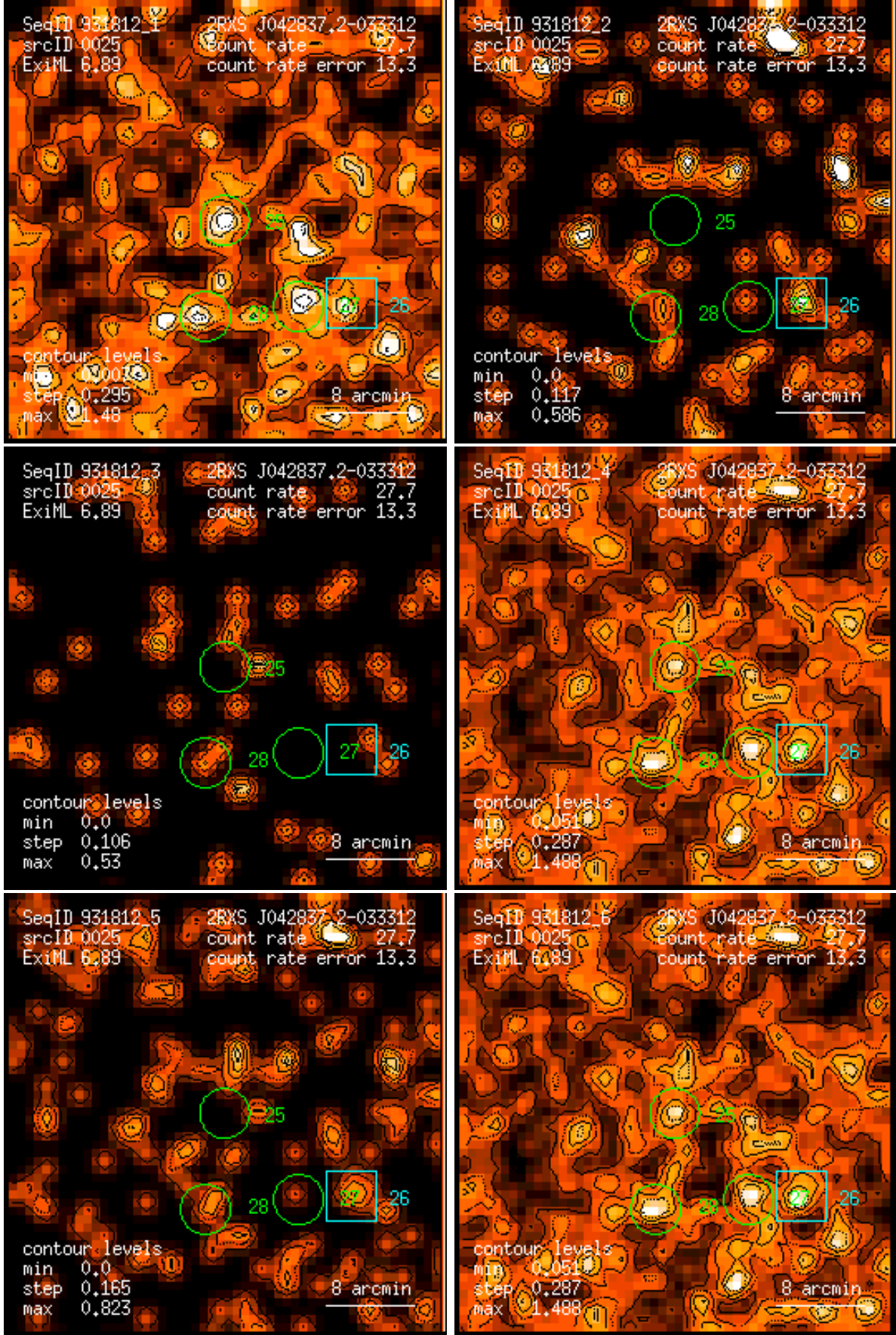
Figure 25: RASS 931812: detection 0025: band rate images, Gaussian filter: (1) PSPC channels 11 – 41, (2) 52 – 90, (3) 91 – 201, (4) 11 – 235, (5) 52 – 201, (6) 11 – 201. Broad band rates in counts/ks. Band rate contour levels in counts/ks/arcmin 2 .
