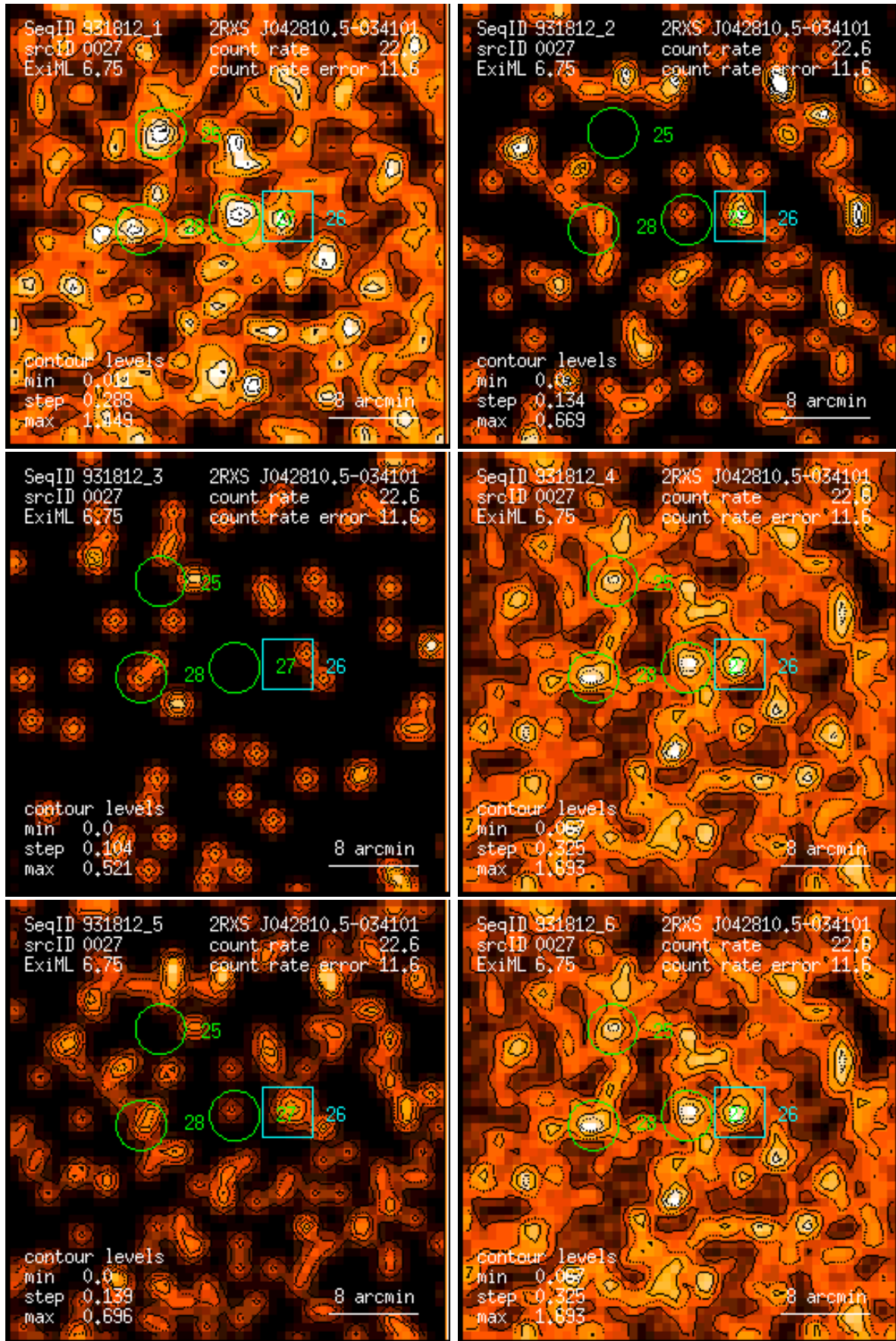
Figure 27: RASS 931812: detection 0027: band rate images, Gaussian filter: (1) PSPC channels 11 – 41, (2) 52 – 90, (3) 91 – 201, (4) 11 – 235, (5) 52 – 201, (6) 11 – 201. Broad band rates in counts/ks. Band rate contour levels in counts/ks/arcmin 2 .
