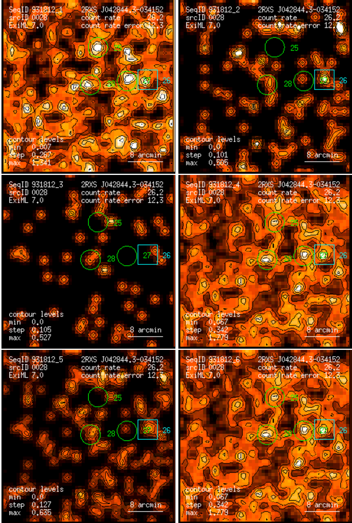
Figure 28: RASS 931812: detection 0028: band rate images, Gaussian filter: (1) PSPC channels 11 – 41, (2) 52 – 90, (3) 91 – 201, (4) 11 – 235, (5) 52 – 201, (6) 11 – 201. Broad band rates in counts/ks. Band rate contour levels in counts/ks/arcmin 2 .
