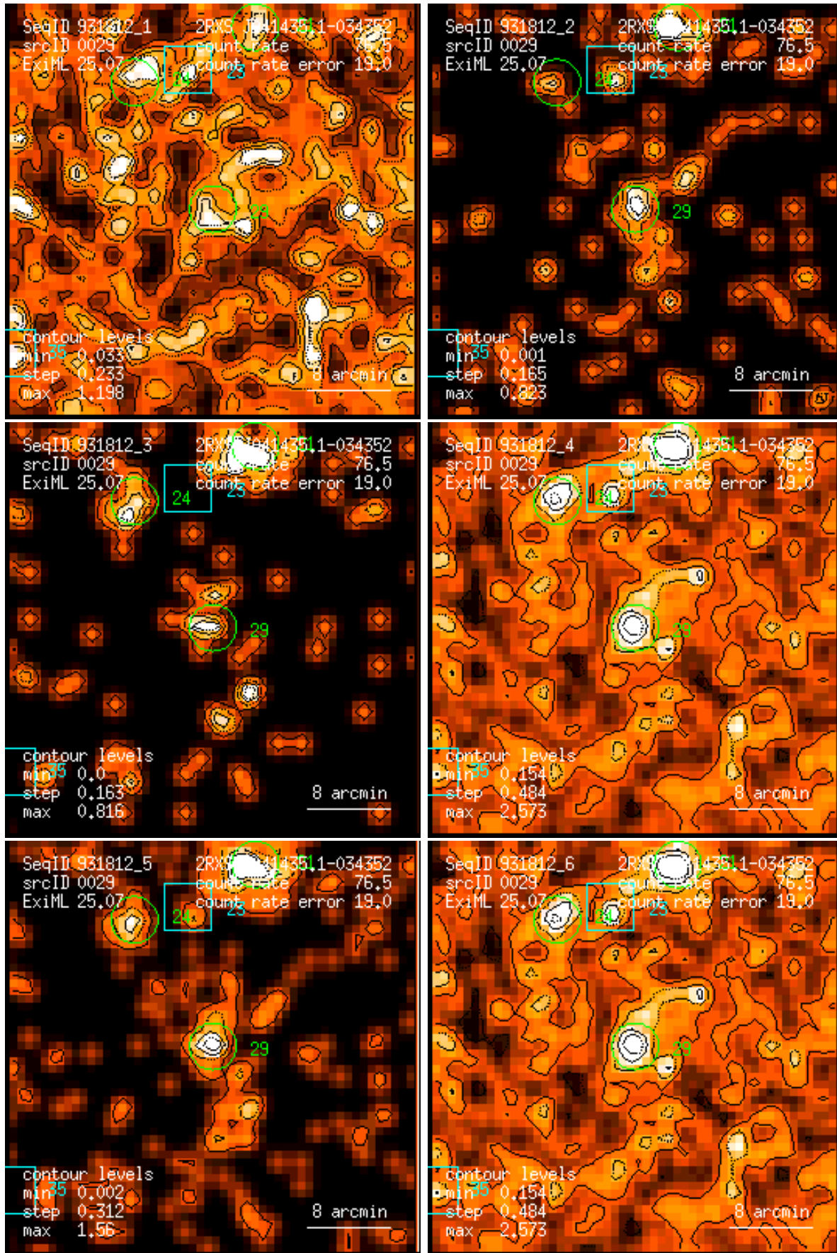
Figure 29: RASS 931812: detection 0029: band rate images, Gaussian filter: (1) PSPC channels 11 – 41, (2) 52 – 90, (3) 91 – 201, (4) 11 – 235, (5) 52 – 201, (6) 11 – 201. Broad band rates in counts/ks. Band rate contour levels in counts/ks/arcmin 2 .
