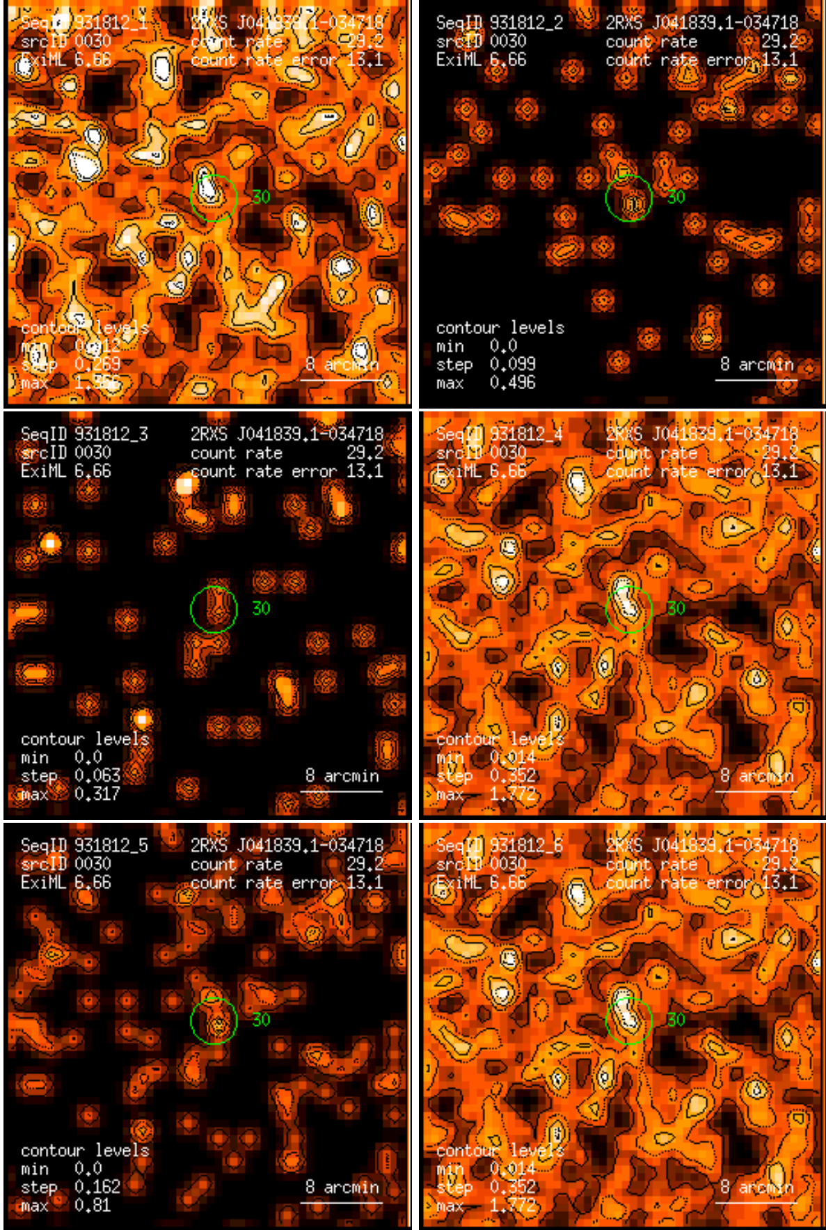
Figure 30: RASS 931812: detection 0030: band rate images, Gaussian filter: (1) PSPC channels 11 – 41, (2) 52 – 90, (3) 91 – 201, (4) 11 – 235, (5) 52 – 201, (6) 11 – 201. Broad band rates in counts/ks. Band rate contour levels in counts/ks/arcmin 2 .
