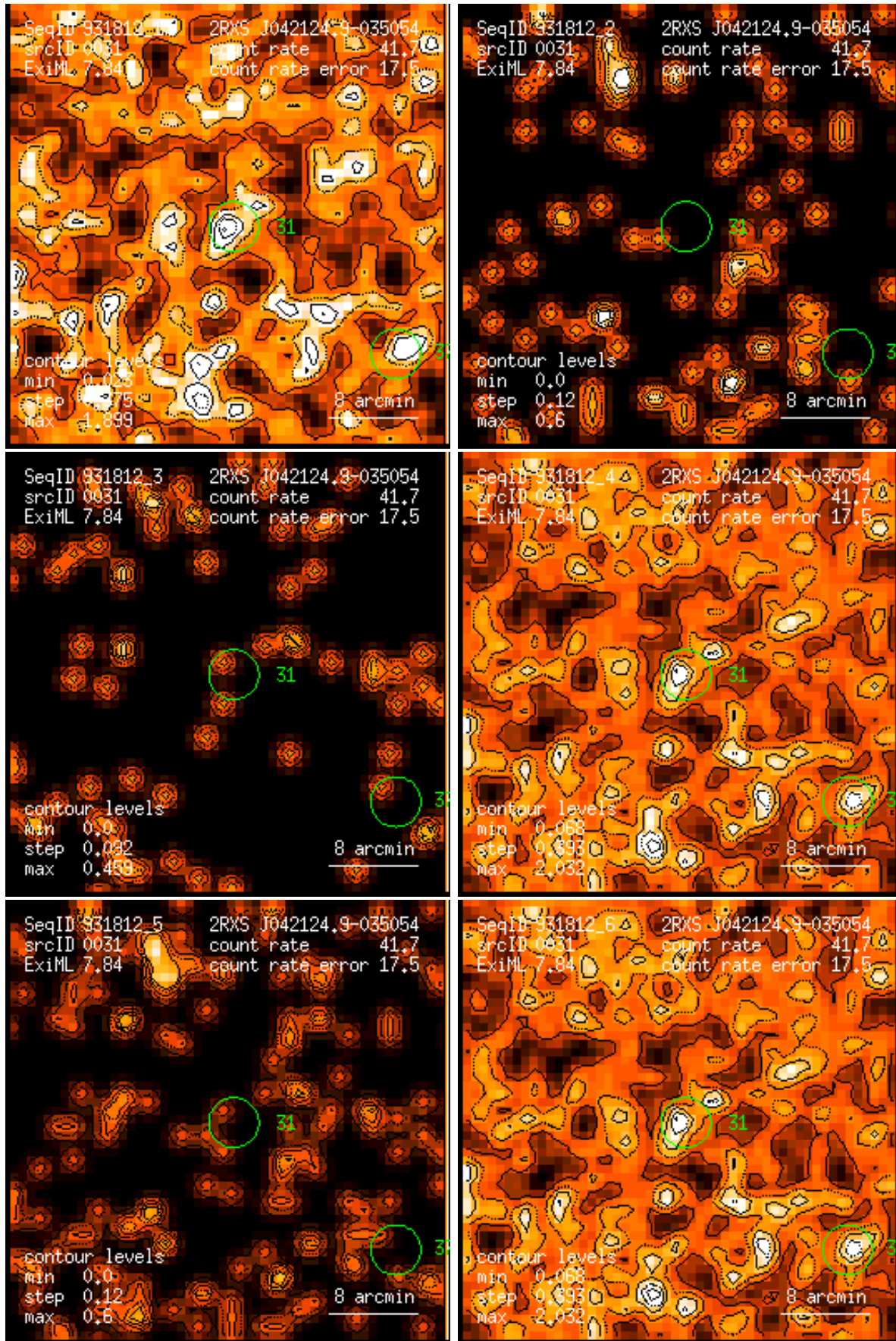
Figure 31: RASS 931812: detection 0031: band rate images, Gaussian filter: (1) PSPC channels 11 – 41, (2) 52 – 90, (3) 91 – 201, (4) 11 – 235, (5) 52 – 201, (6) 11 – 201. Broad band rates in counts/ks. Band rate contour levels in counts/ks/arcmin 2 .
