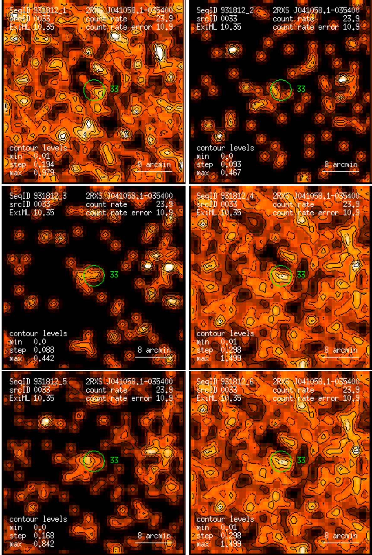
Figure 33: RASS 931812: detection 0033: band rate images, Gaussian filter: (1) PSPC channels 11 – 41, (2) 52 – 90, (3) 91 – 201, (4) 11 – 235, (5) 52 – 201, (6) 11 – 201. Broad band rates in counts/ks. Band rate contour levels in counts/ks/arcmin 2 .
