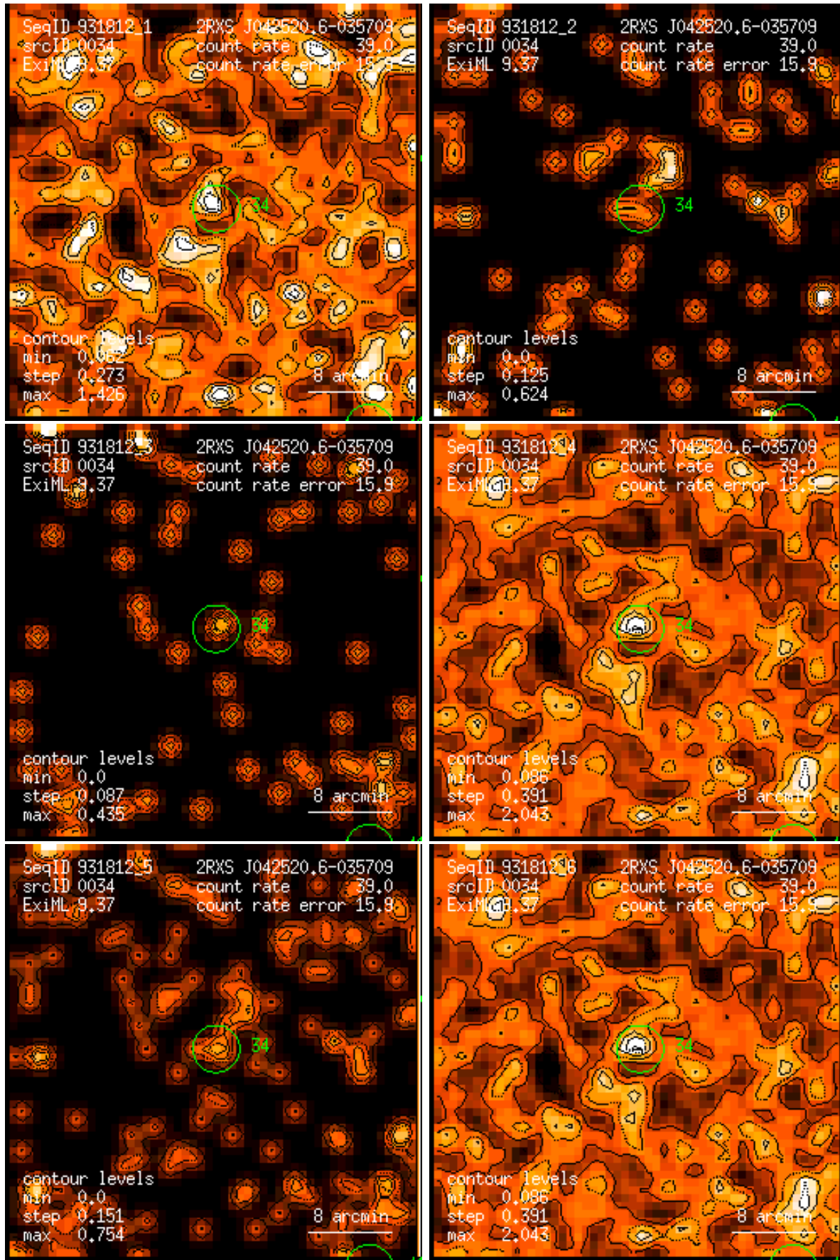
Figure 34: RASS 931812: detection 0034: band rate images, Gaussian filter: (1) PSPC channels 11 – 41, (2) 52 – 90, (3) 91 – 201, (4) 11 – 235, (5) 52 – 201, (6) 11 – 201. Broad band rates in counts/ks. Band rate contour levels in counts/ks/arcmin 2 .
