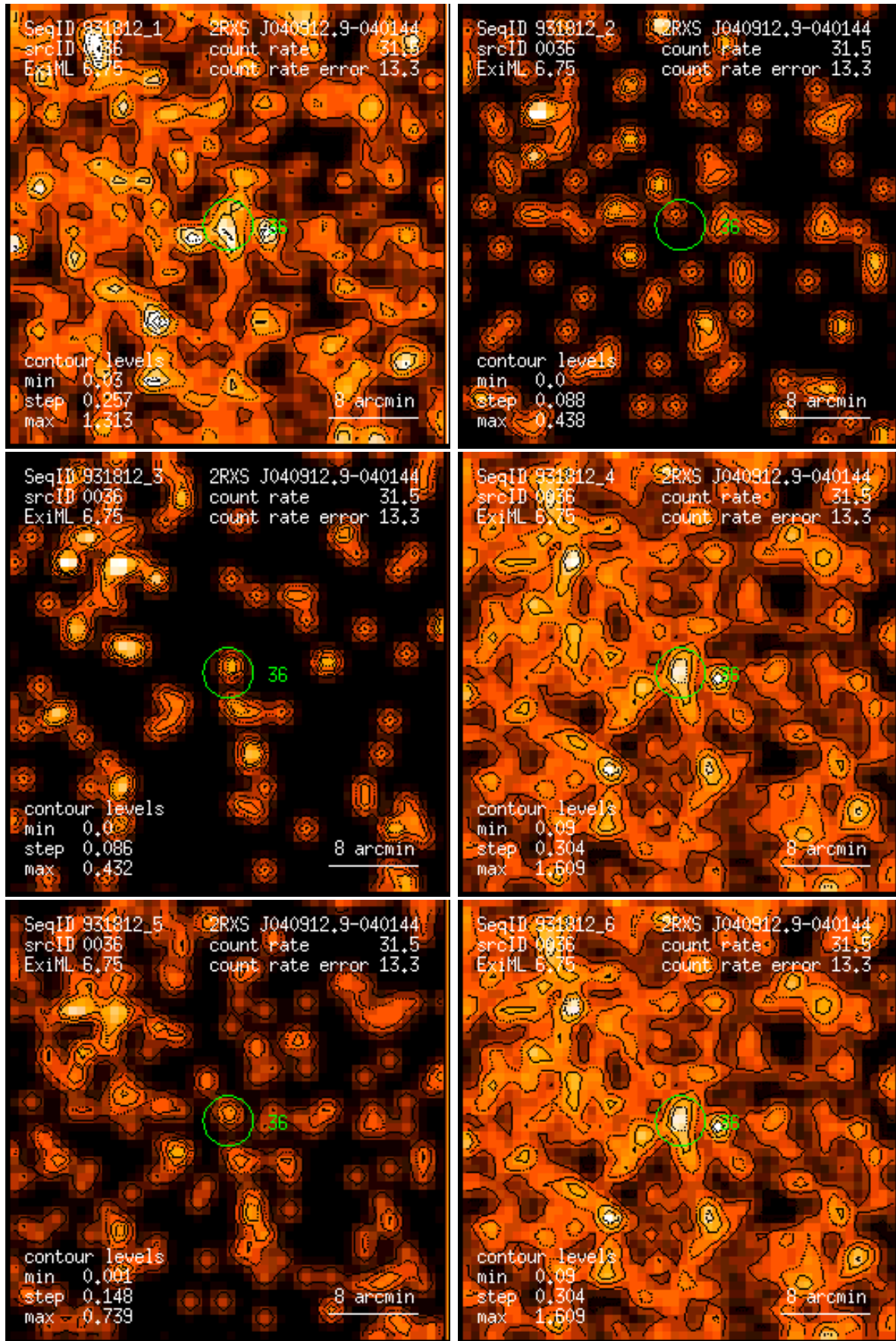
Figure 36: RASS 931812: detection 0036: band rate images, Gaussian filter: (1) PSPC channels 11 – 41, (2) 52 – 90, (3) 91 – 201, (4) 11 – 235, (5) 52 – 201, (6) 11 – 201. Broad band rates in counts/ks. Band rate contour levels in counts/ks/arcmin 2 .
