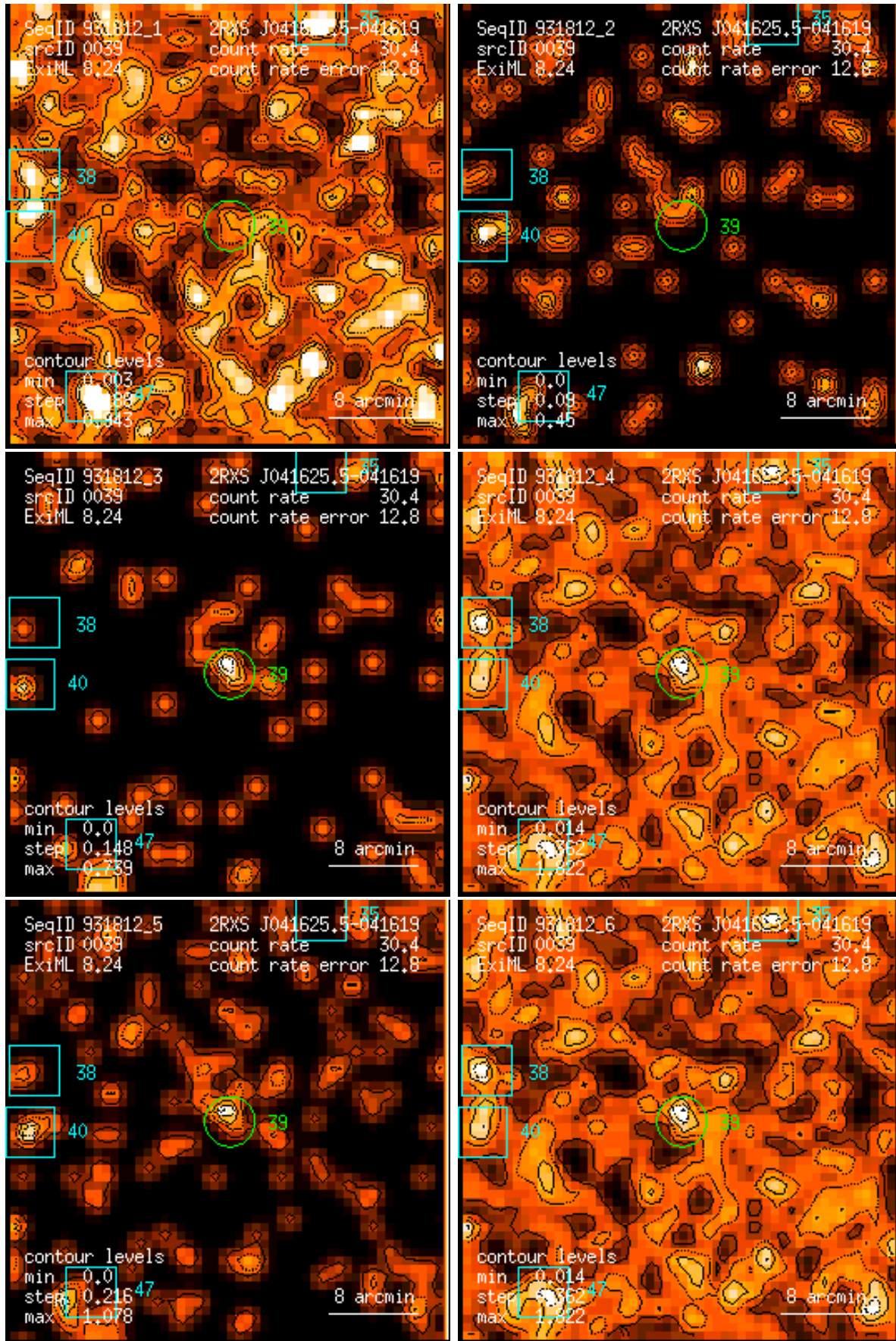
Figure 39: RASS 931812: detection 0039: band rate images, Gaussian filter: (1) PSPC channels 11 – 41, (2) 52 – 90, (3) 91 – 201, (4) 11 – 235, (5) 52 – 201, (6) 11 – 201. Broad band rates in counts/ks. Band rate contour levels in counts/ks/arcmin 2 .
