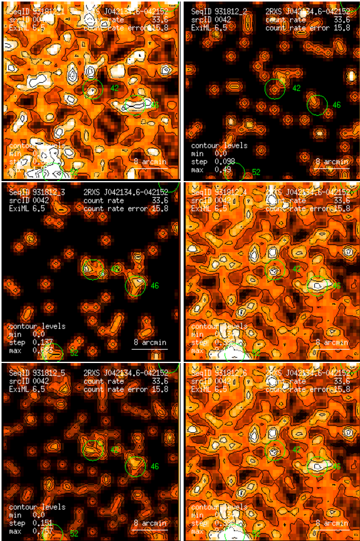
Figure 42: RASS 931812: detection 0042: band rate images, Gaussian filter: (1) PSPC channels 11 – 41, (2) 52 – 90, (3) 91 – 201, (4) 11 – 235, (5) 52 – 201, (6) 11 – 201. Broad band rates in counts/ks. Band rate contour levels in counts/ks/arcmin 2 .
