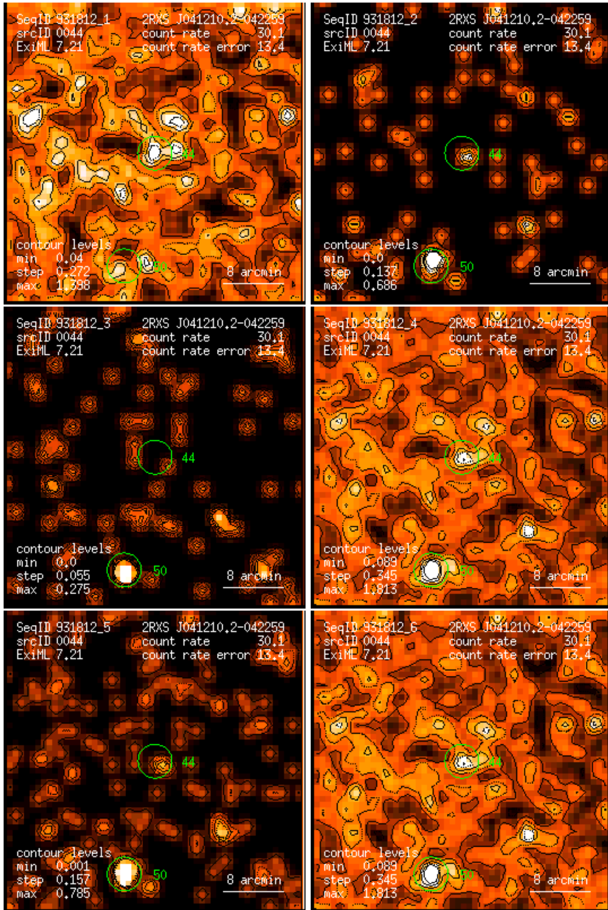
Figure 44: RASS 931812: detection 0044: band rate images, Gaussian filter: (1) PSPC channels 11 – 41, (2) 52 – 90, (3) 91 – 201, (4) 11 – 235, (5) 52 – 201, (6) 11 – 201. Broad band rates in counts/ks. Band rate contour levels in counts/ks/arcmin 2 .
