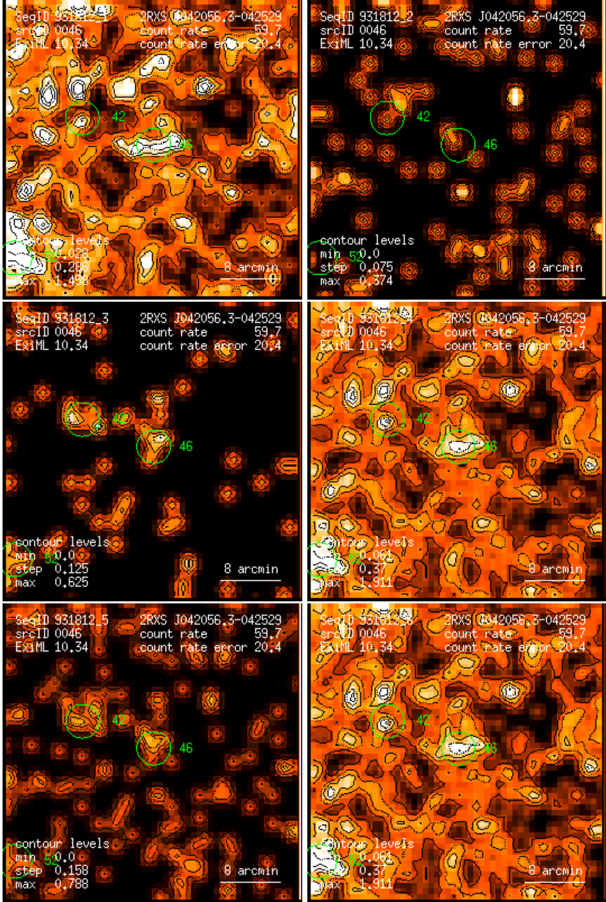
Figure 46: RASS 931812: detection 0046: band rate images, Gaussian filter: (1) PSPC channels 11 – 41, (2) 52 – 90, (3) 91 – 201, (4) 11 – 235, (5) 52 – 201, (6) 11 – 201. Broad band rates in counts/ks. Band rate contour levels in counts/ks/arcmin 2 .
