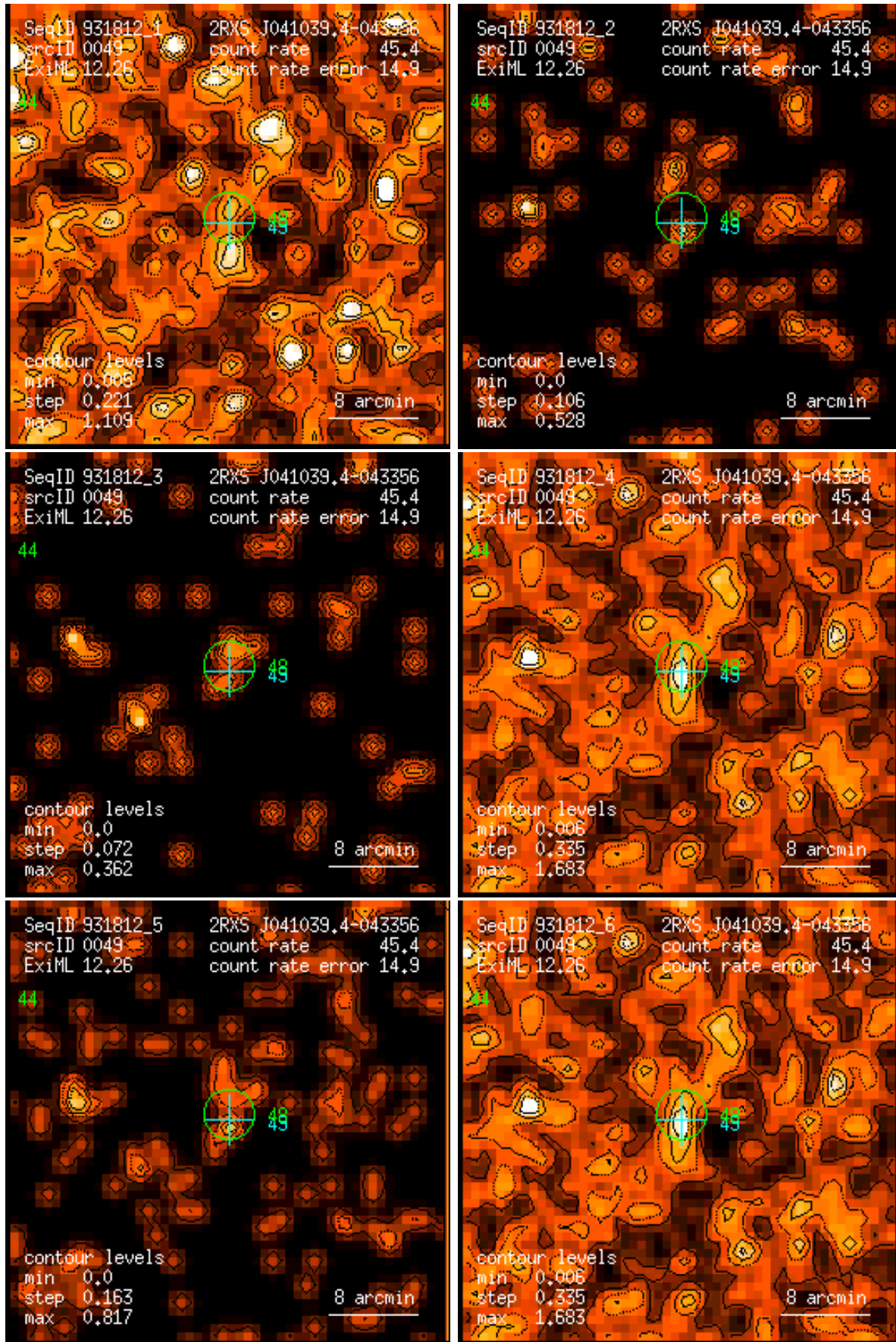
Figure 49: RASS 931812: detection 0049: band rate images, Gaussian filter: (1) PSPC channels 11 – 41, (2) 52 – 90, (3) 91 – 201, (4) 11 – 235, (5) 52 – 201, (6) 11 – 201. Broad band rates in counts/ks. Band rate contour levels in counts/ks/arcmin 2 .
