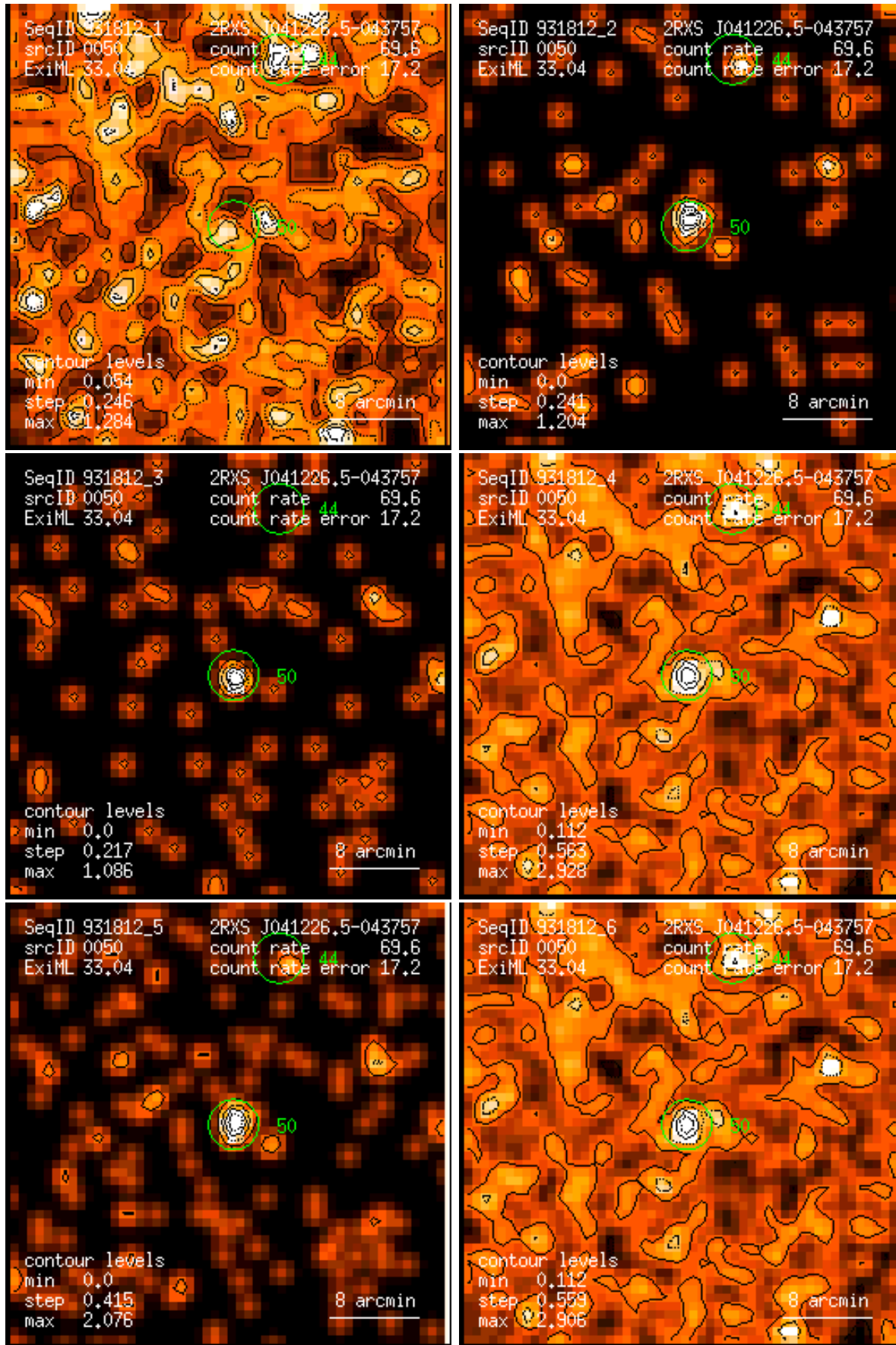
Figure 50: RASS 931812: detection 0050: band rate images, Gaussian filter: (1) PSPC channels 11 – 41, (2) 52 – 90, (3) 91 – 201, (4) 11 – 235, (5) 52 – 201, (6) 11 – 201. Broad band rates in counts/ks. Band rate contour levels in counts/ks/arcmin 2 .
