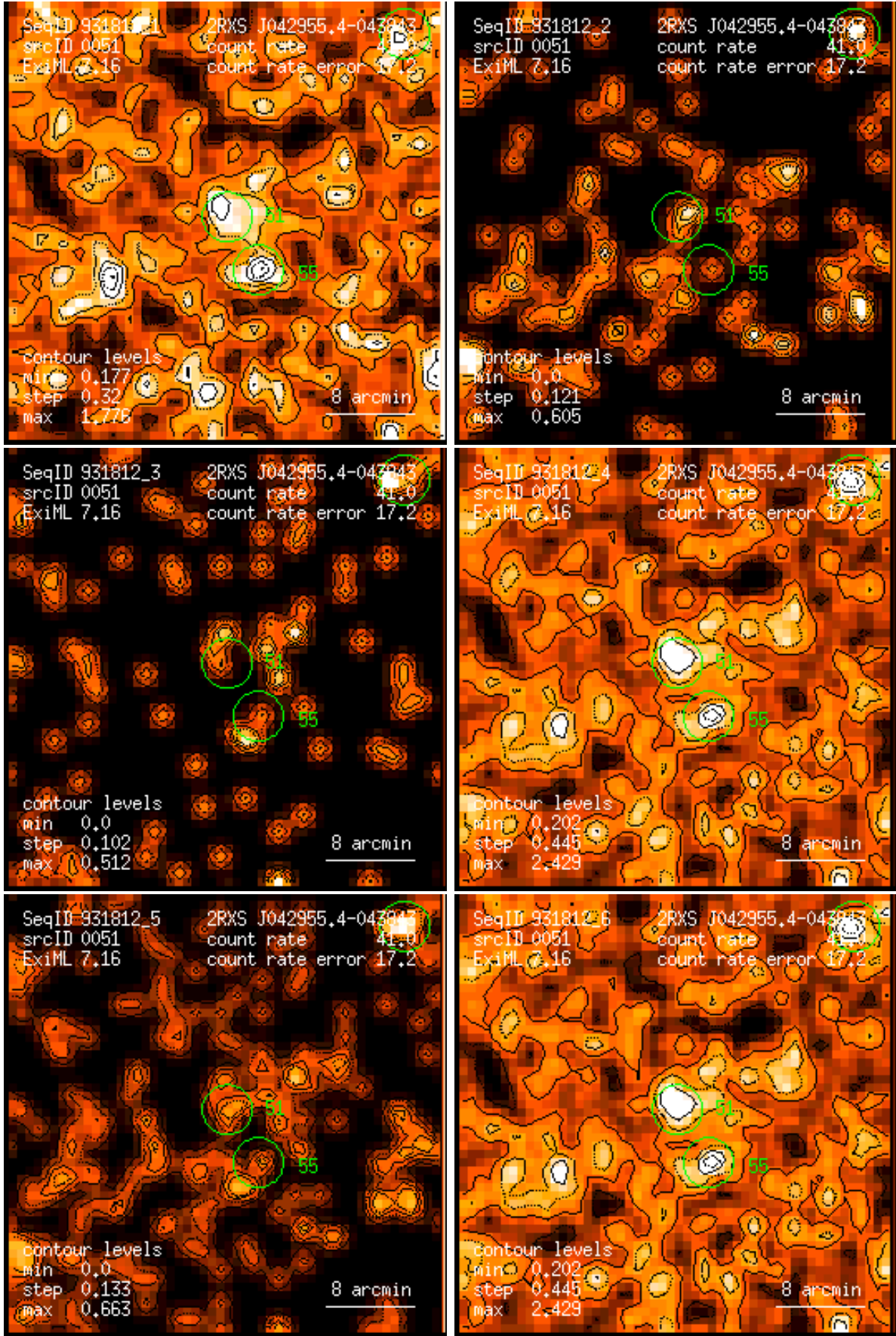
Figure 51: RASS 931812: detection 0051: band rate images, Gaussian filter: (1) PSPC channels 11 – 41, (2) 52 – 90, (3) 91 – 201, (4) 11 – 235, (5) 52 – 201, (6) 11 – 201. Broad band rates in counts/ks. Band rate contour levels in counts/ks/arcmin 2 .
