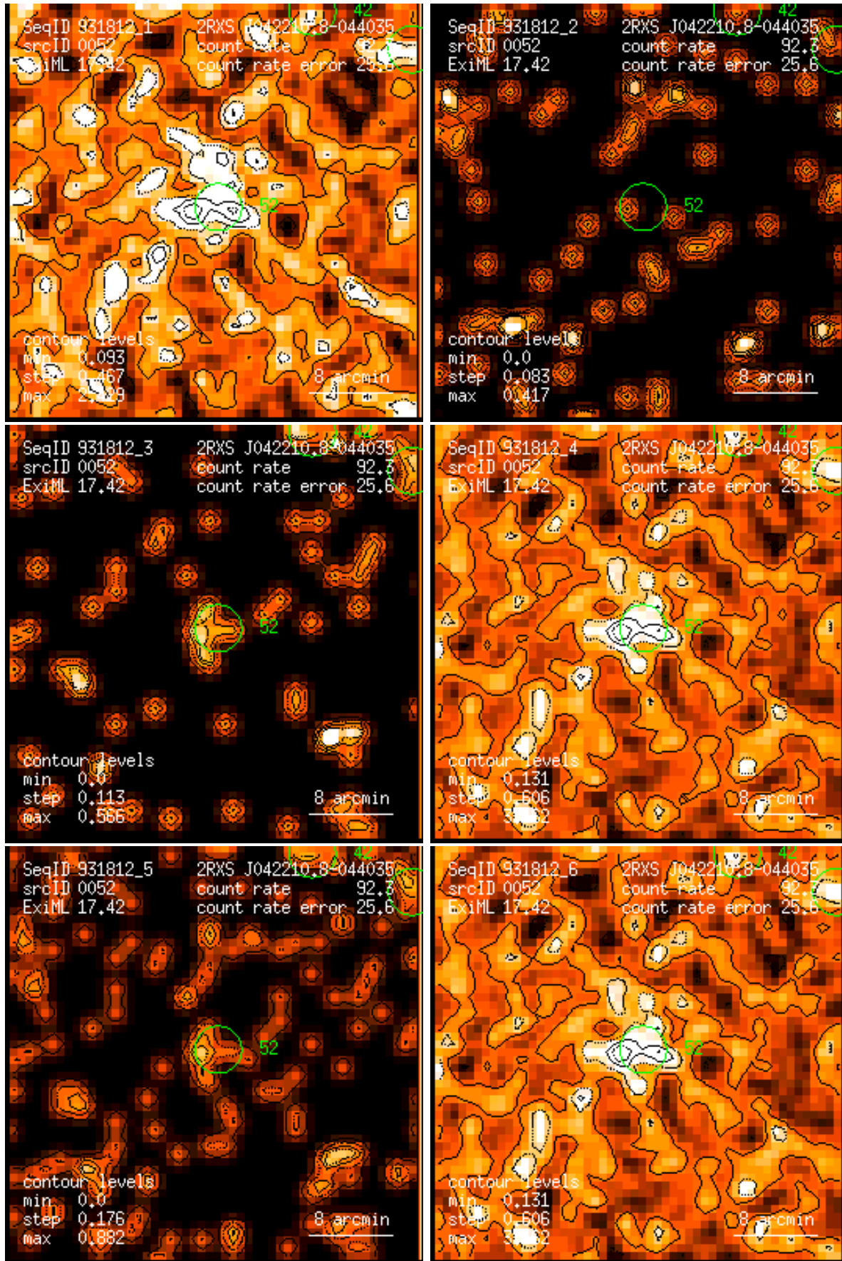
Figure 52: RASS 931812: detection 0052: band rate images, Gaussian filter: (1) PSPC channels 11 – 41, (2) 52 – 90, (3) 91 – 201, (4) 11 – 235, (5) 52 – 201, (6) 11 – 201. Broad band rates in counts/ks. Band rate contour levels in counts/ks/arcmin 2 .
