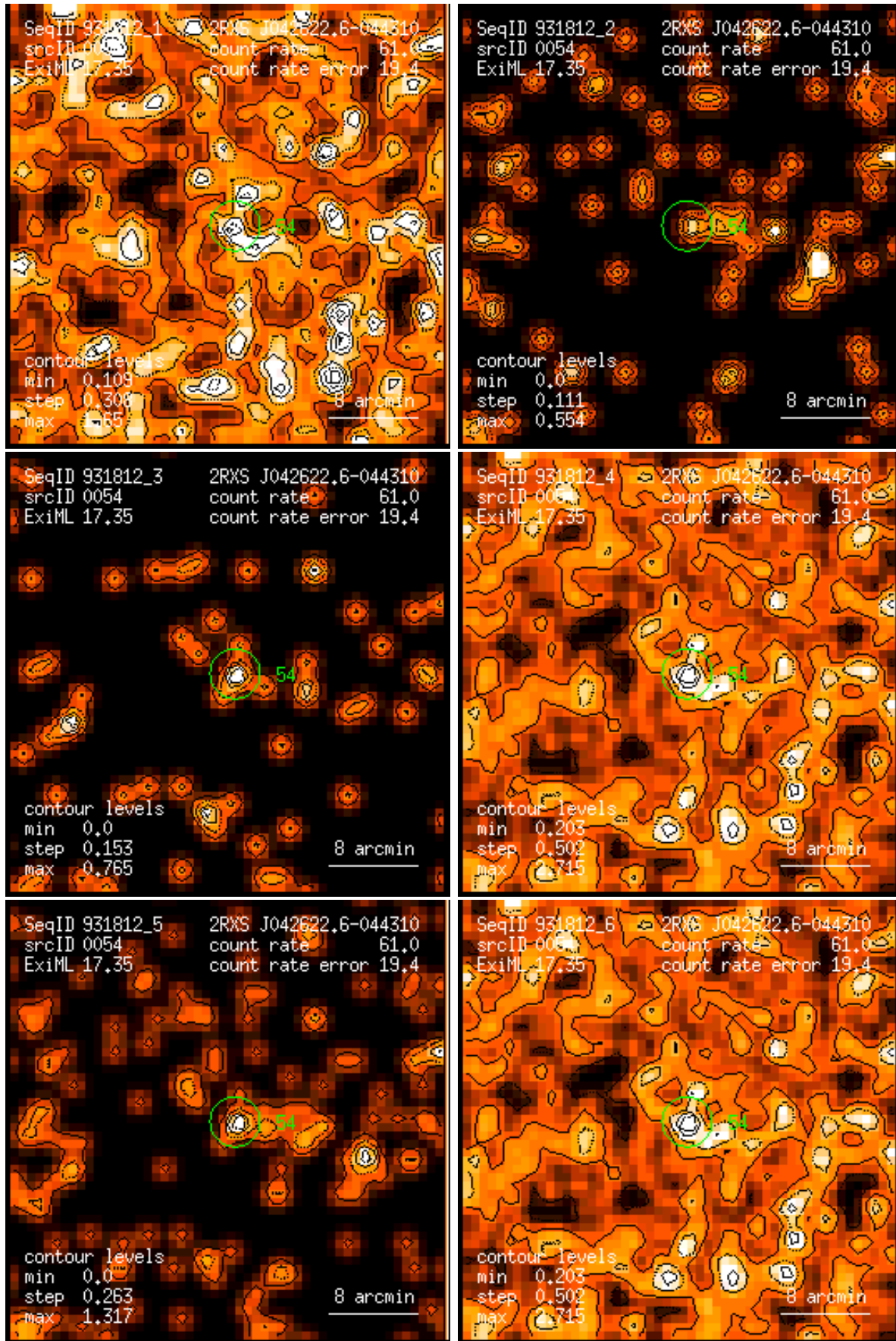
Figure 54: RASS 931812: detection 0054: band rate images, Gaussian filter: (1) PSPC channels 11 – 41, (2) 52 – 90, (3) 91 – 201, (4) 11 – 235, (5) 52 – 201, (6) 11 – 201. Broad band rates in counts/ks. Band rate contour levels in counts/ks/arcmin 2 .
