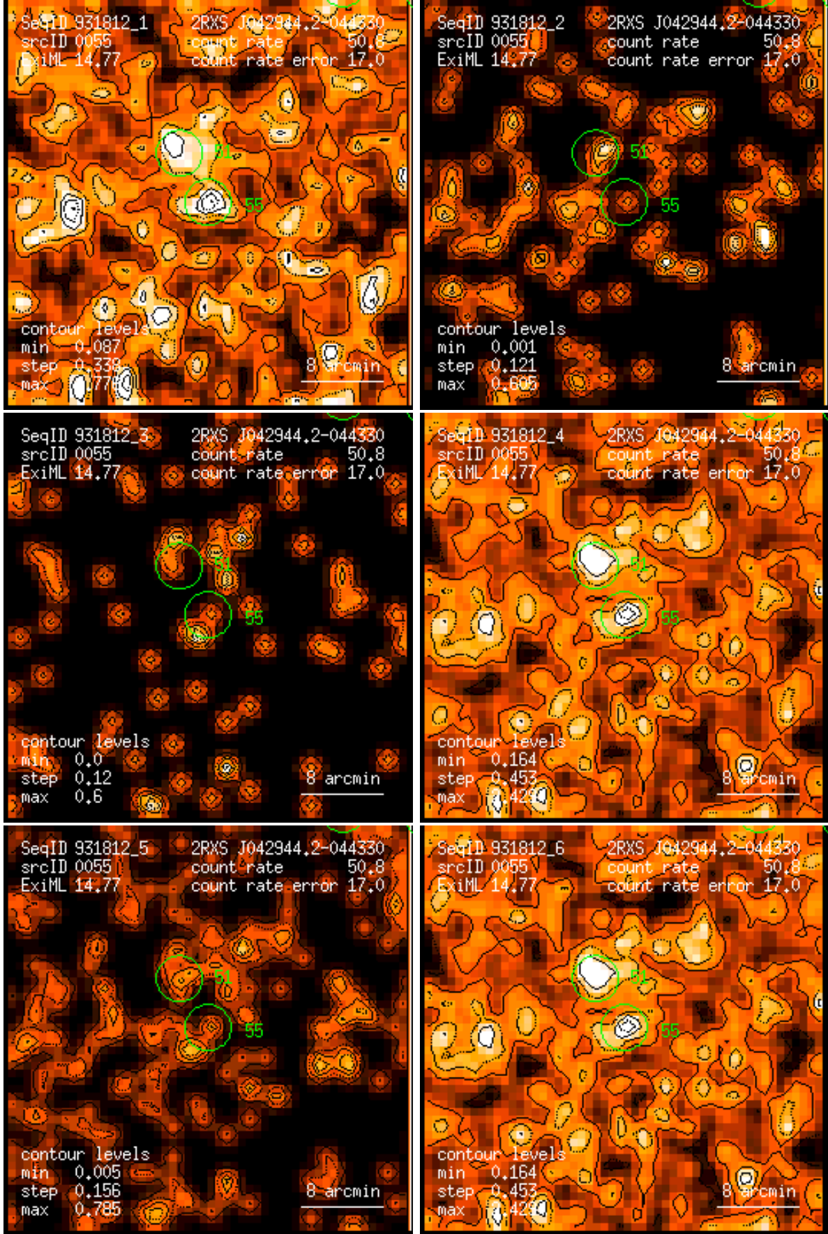
Figure 55: RASS 931812: detection 0055: band rate images, Gaussian filter: (1) PSPC channels 11 – 41, (2) 52 – 90, (3) 91 – 201, (4) 11 – 235, (5) 52 – 201, (6) 11 – 201. Broad band rates in counts/ks. Band rate contour levels in counts/ks/arcmin 2 .
