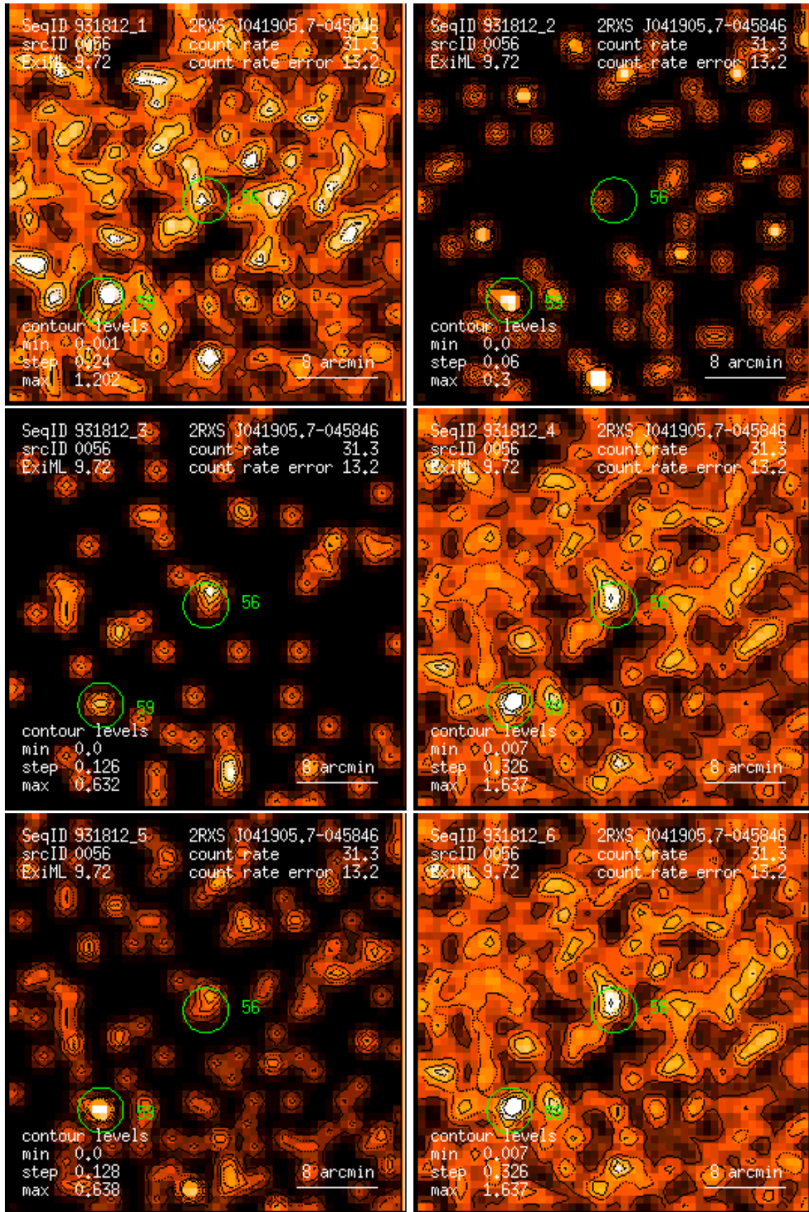
Figure 56: RASS 931812: detection 0056: band rate images, Gaussian filter: (1) PSPC channels 11 – 41, (2) 52 – 90, (3) 91 – 201, (4) 11 – 235, (5) 52 – 201, (6) 11 – 201. Broad band rates in counts/ks. Band rate contour levels in counts/ks/arcmin 2 .
