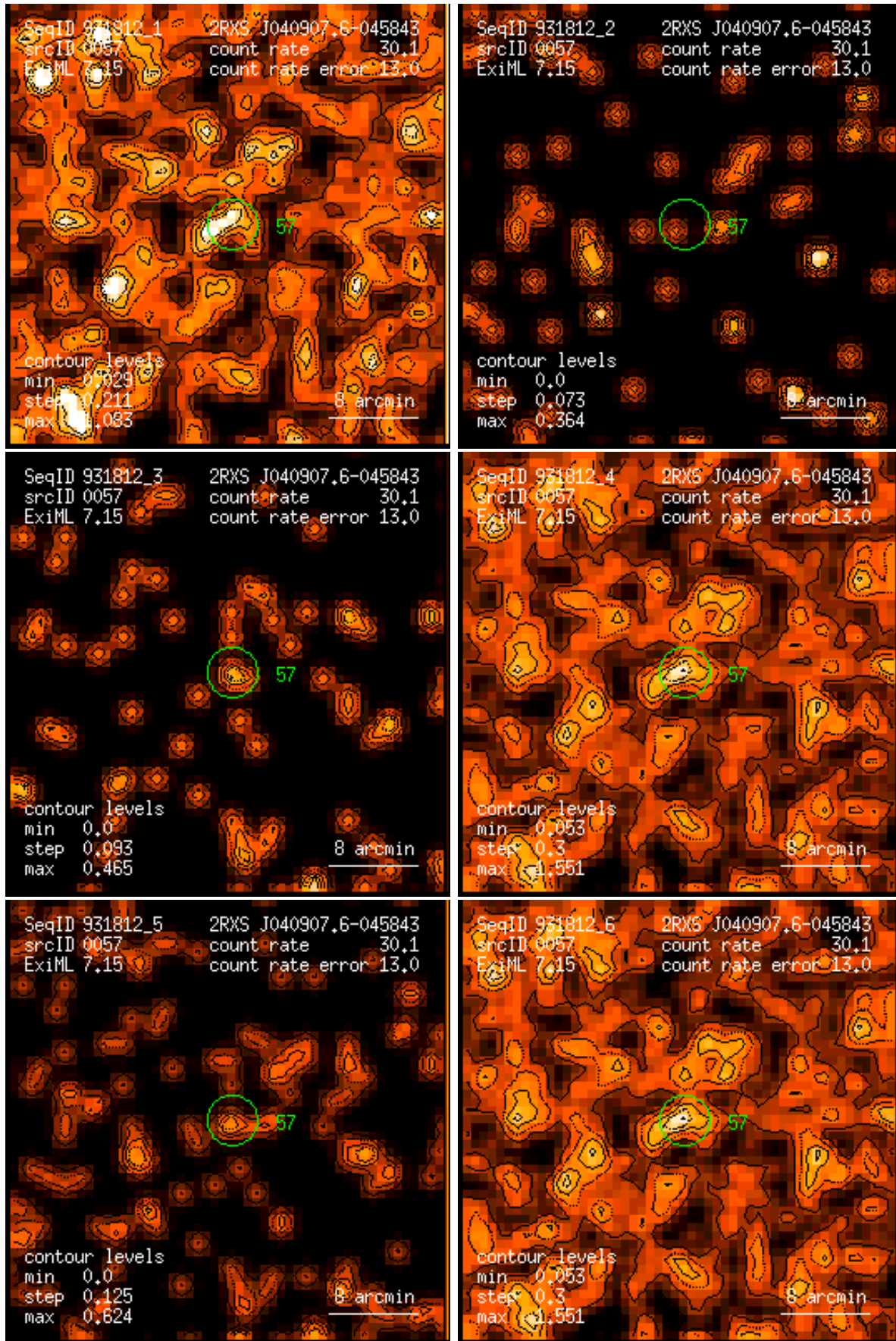
Figure 57: RASS 931812: detection 0057: band rate images, Gaussian filter: (1) PSPC channels 11 – 41, (2) 52 – 90, (3) 91 – 201, (4) 11 – 235, (5) 52 – 201, (6) 11 – 201. Broad band rates in counts/ks. Band rate contour levels in counts/ks/arcmin 2 .
