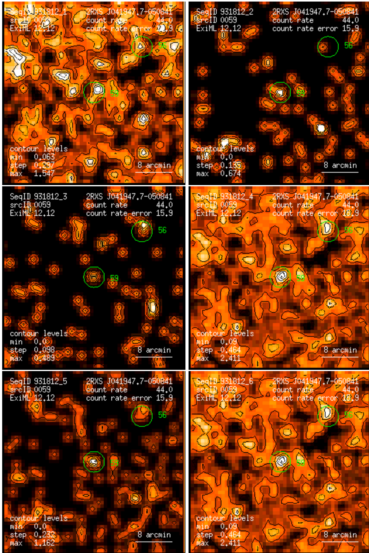
Figure 59: RASS 931812: detection 0059: band rate images, Gaussian filter: (1) PSPC channels 11 – 41, (2) 52 – 90, (3) 91 – 201, (4) 11 – 235, (5) 52 – 201, (6) 11 – 201. Broad band rates in counts/ks. Band rate contour levels in counts/ks/arcmin 2 .
