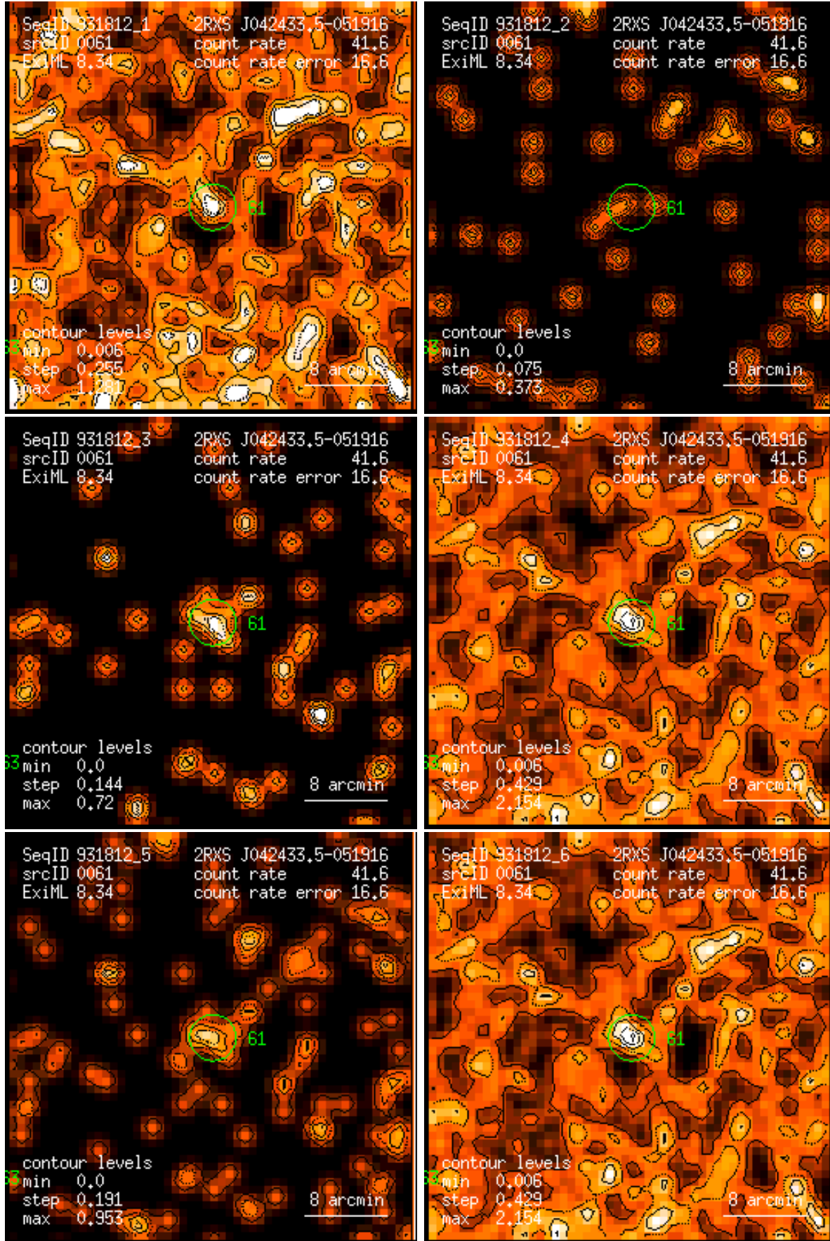
Figure 61: RASS 931812: detection 0061: band rate images, Gaussian filter: (1) PSPC channels 11 – 41, (2) 52 – 90, (3) 91 – 201, (4) 11 – 235, (5) 52 – 201, (6) 11 – 201. Broad band rates in counts/ks. Band rate contour levels in counts/ks/arcmin 2 .
