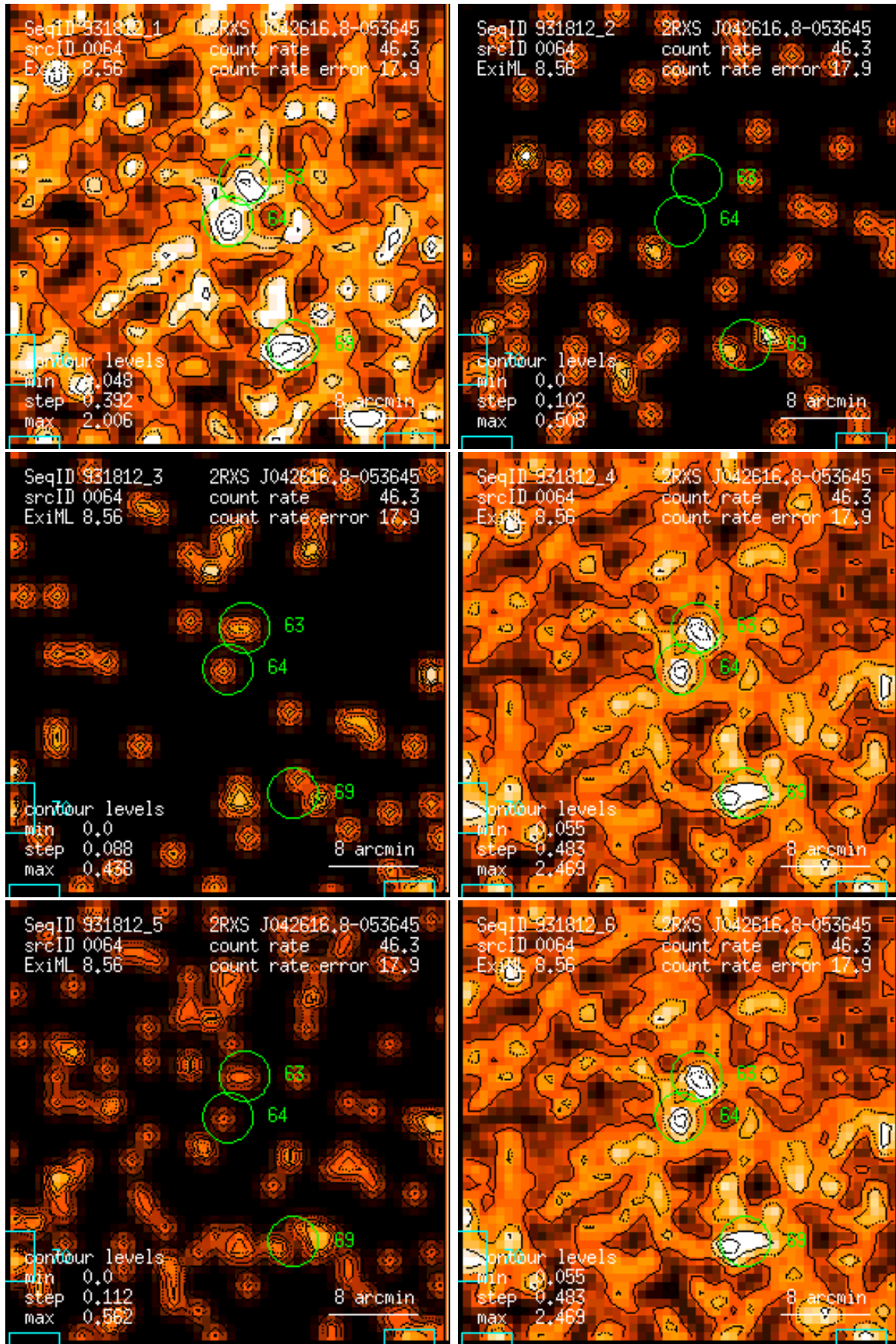
Figure 64: RASS 931812: detection 0064: band rate images, Gaussian filter: (1) PSPC channels 11 – 41, (2) 52 – 90, (3) 91 – 201, (4) 11 – 235, (5) 52 – 201, (6) 11 – 201. Broad band rates in counts/ks. Band rate contour levels in counts/ks/arcmin 2 .
