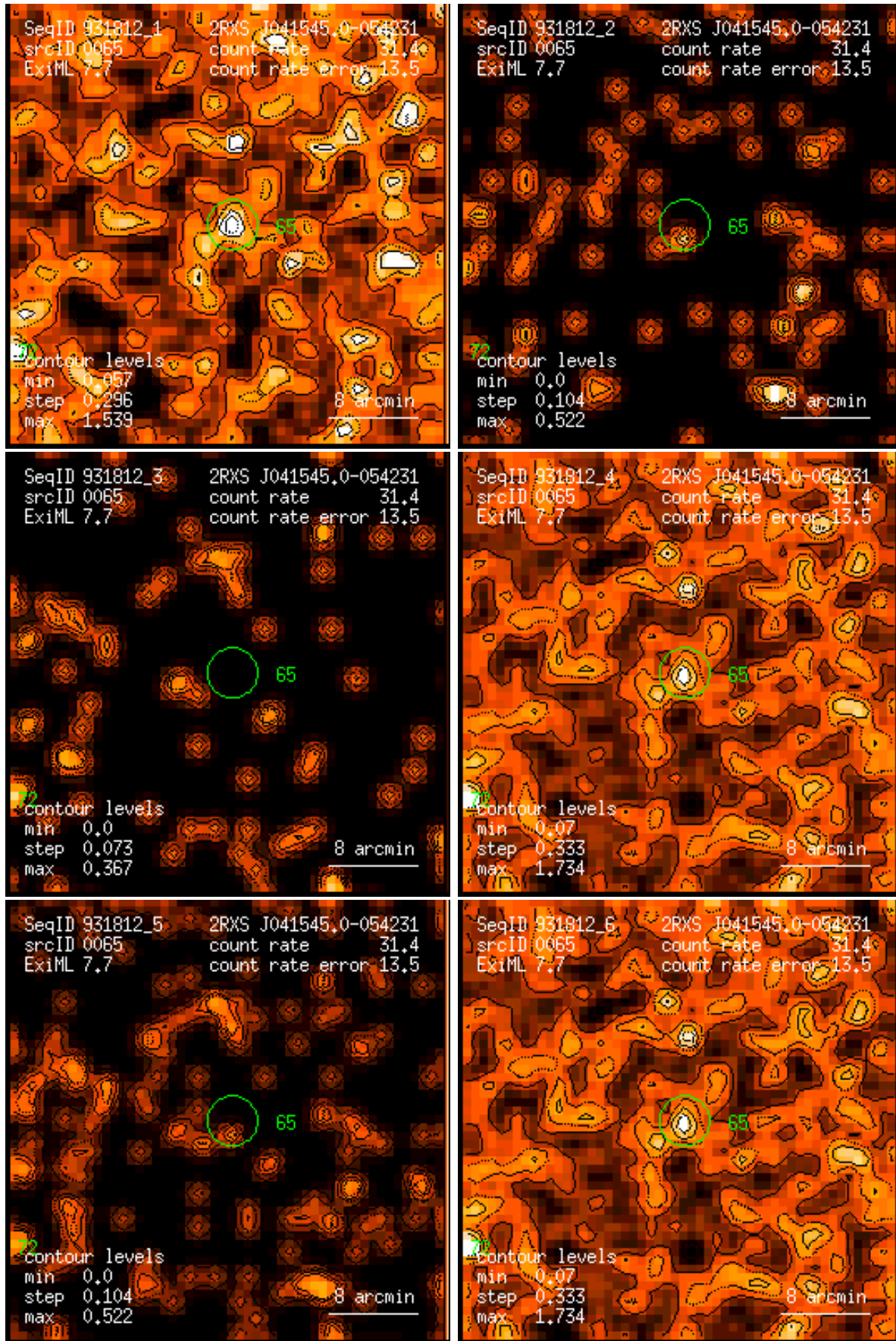
Figure 65: RASS 931812: detection 0065: band rate images, Gaussian filter: (1) PSPC channels 11 – 41, (2) 52 – 90, (3) 91 – 201, (4) 11 – 235, (5) 52 – 201, (6) 11 – 201. Broad band rates in counts/ks. Band rate contour levels in counts/ks/arcmin 2 .
