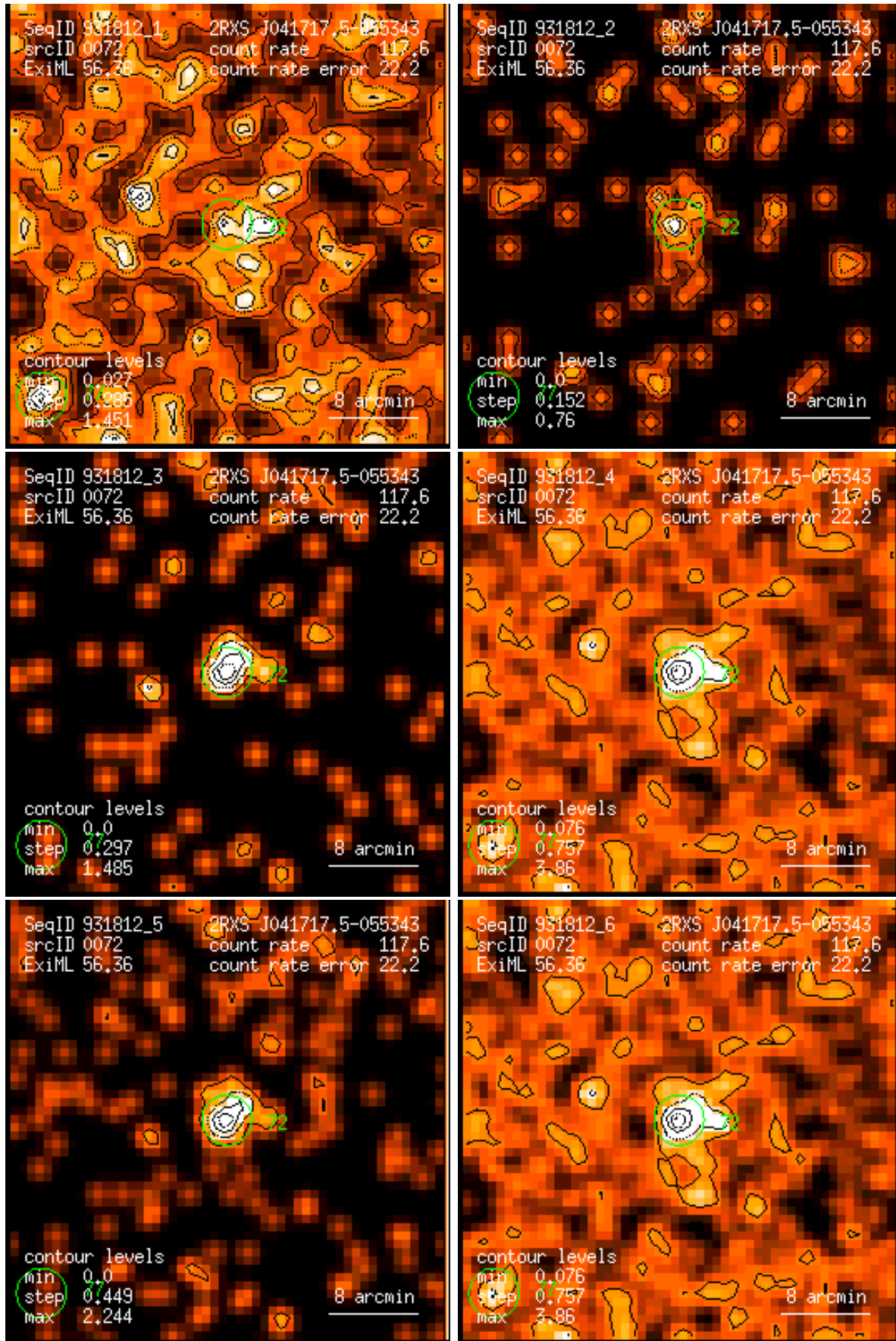
Figure 72: RASS 931812: detection 0072: band rate images, Gaussian filter: (1) PSPC channels 11 – 41, (2) 52 – 90, (3) 91 – 201, (4) 11 – 235, (5) 52 – 201, (6) 11 – 201. Broad band rates in counts/ks. Band rate contour levels in counts/ks/arcmin 2 .
