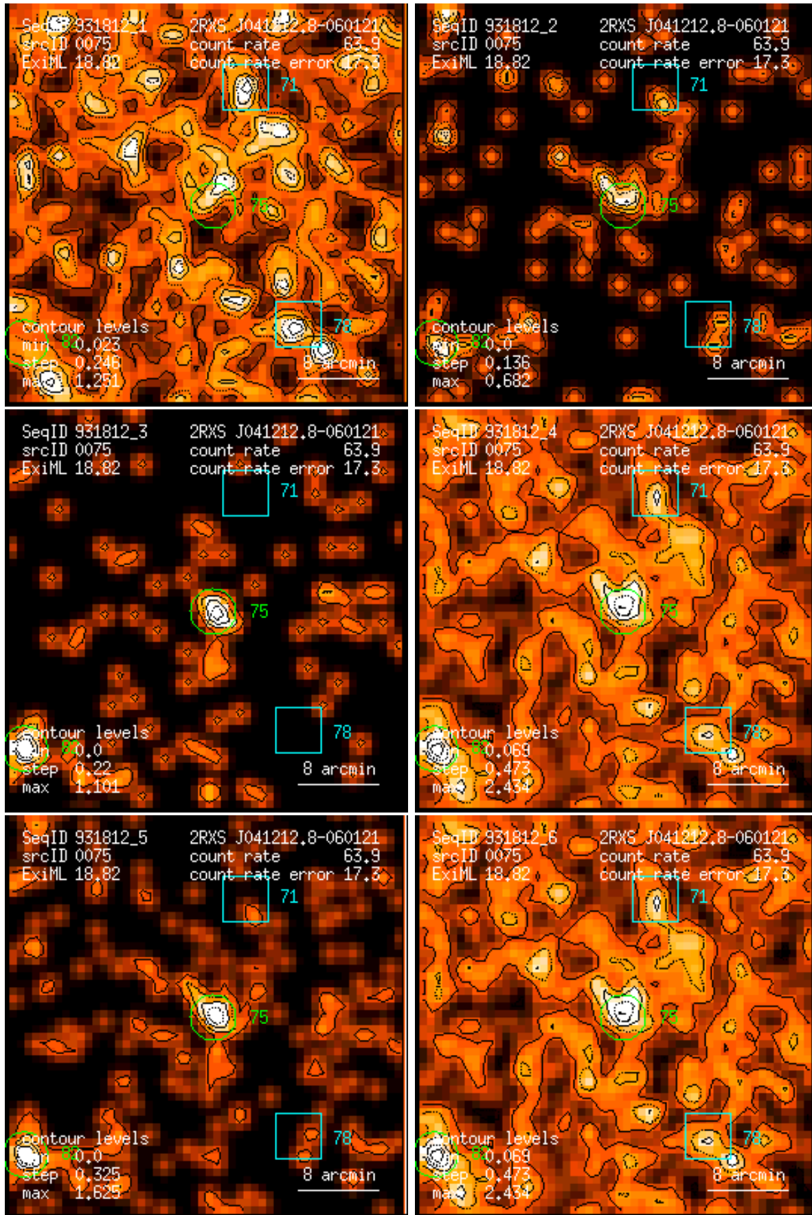
Figure 75: RASS 931812: detection 0075: band rate images, Gaussian filter: (1) PSPC channels 11 – 41, (2) 52 – 90, (3) 91 – 201, (4) 11 – 235, (5) 52 – 201, (6) 11 – 201. Broad band rates in counts/ks. Band rate contour levels in counts/ks/arcmin 2 .
