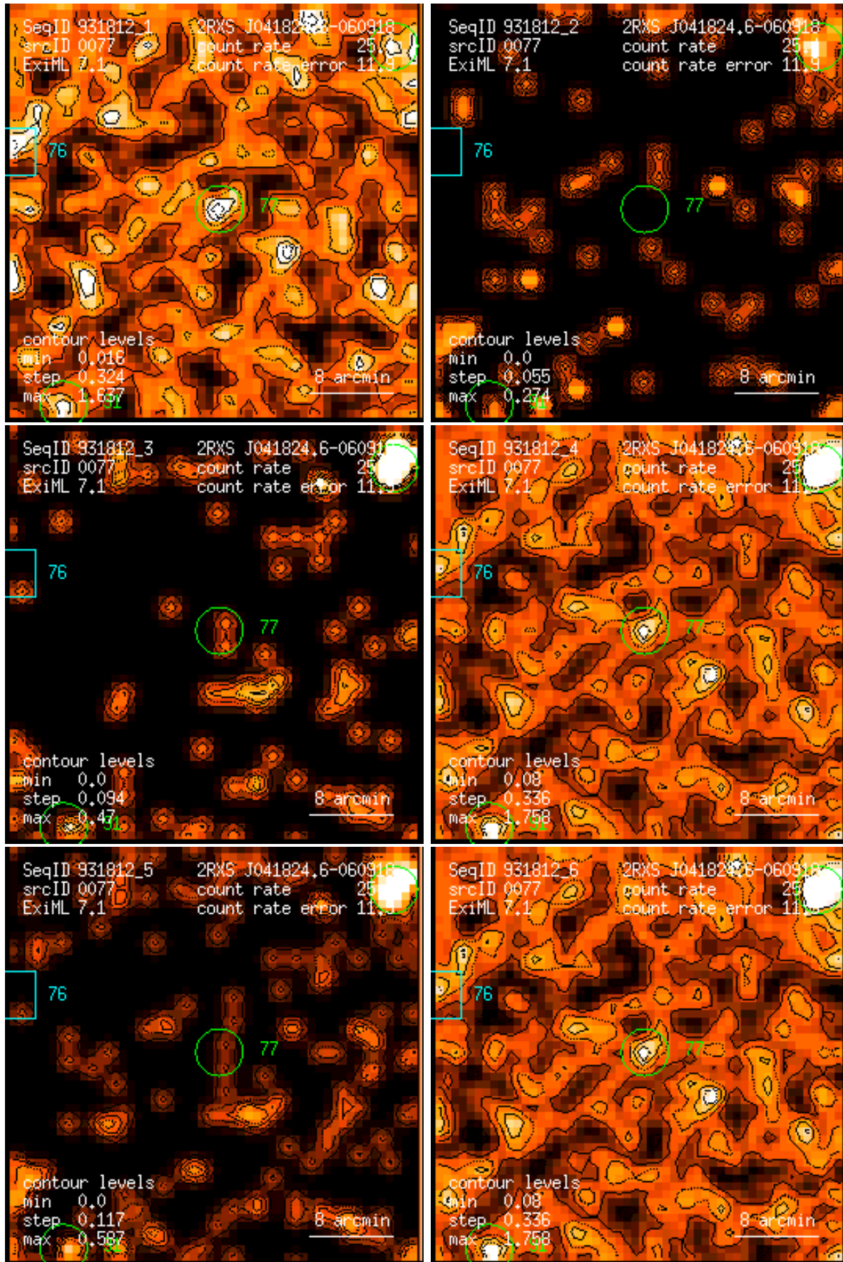
Figure 77: RASS 931812: detection 0077: band rate images, Gaussian filter: (1) PSPC channels 11 – 41, (2) 52 – 90, (3) 91 – 201, (4) 11 – 235, (5) 52 – 201, (6) 11 – 201. Broad band rates in counts/ks. Band rate contour levels in counts/ks/arcmin 2 .
