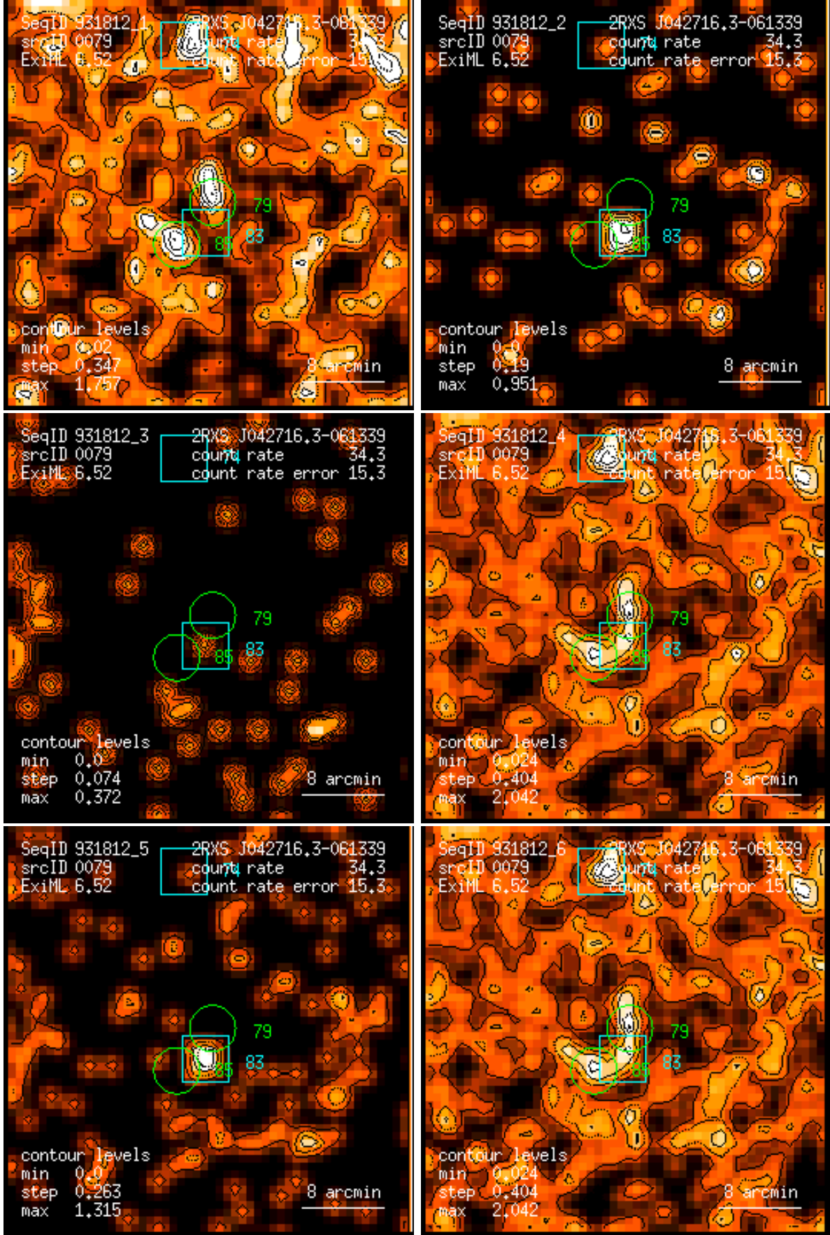
Figure 79: RASS 931812: detection 0079: band rate images, Gaussian filter: (1) PSPC channels 11 – 41, (2) 52 – 90, (3) 91 – 201, (4) 11 – 235, (5) 52 – 201, (6) 11 – 201. Broad band rates in counts/ks. Band rate contour levels in counts/ks/arcmin 2 .
