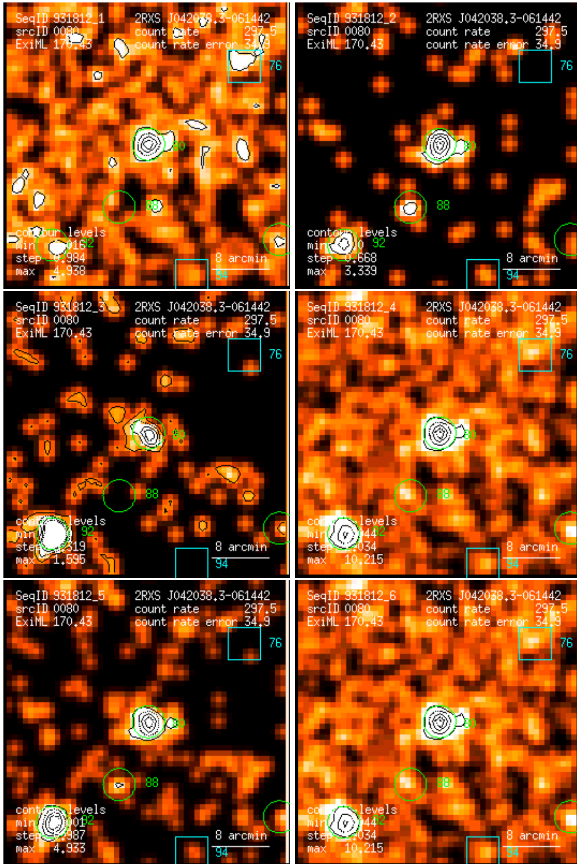
Figure 80: RASS 931812: detection 0080: band rate images, Gaussian filter: (1) PSPC channels 11 – 41, (2) 52 – 90, (3) 91 – 201, (4) 11 – 235, (5) 52 – 201, (6) 11 – 201. Broad band rates in counts/ks. Band rate contour levels in counts/ks/arcmin 2 .
