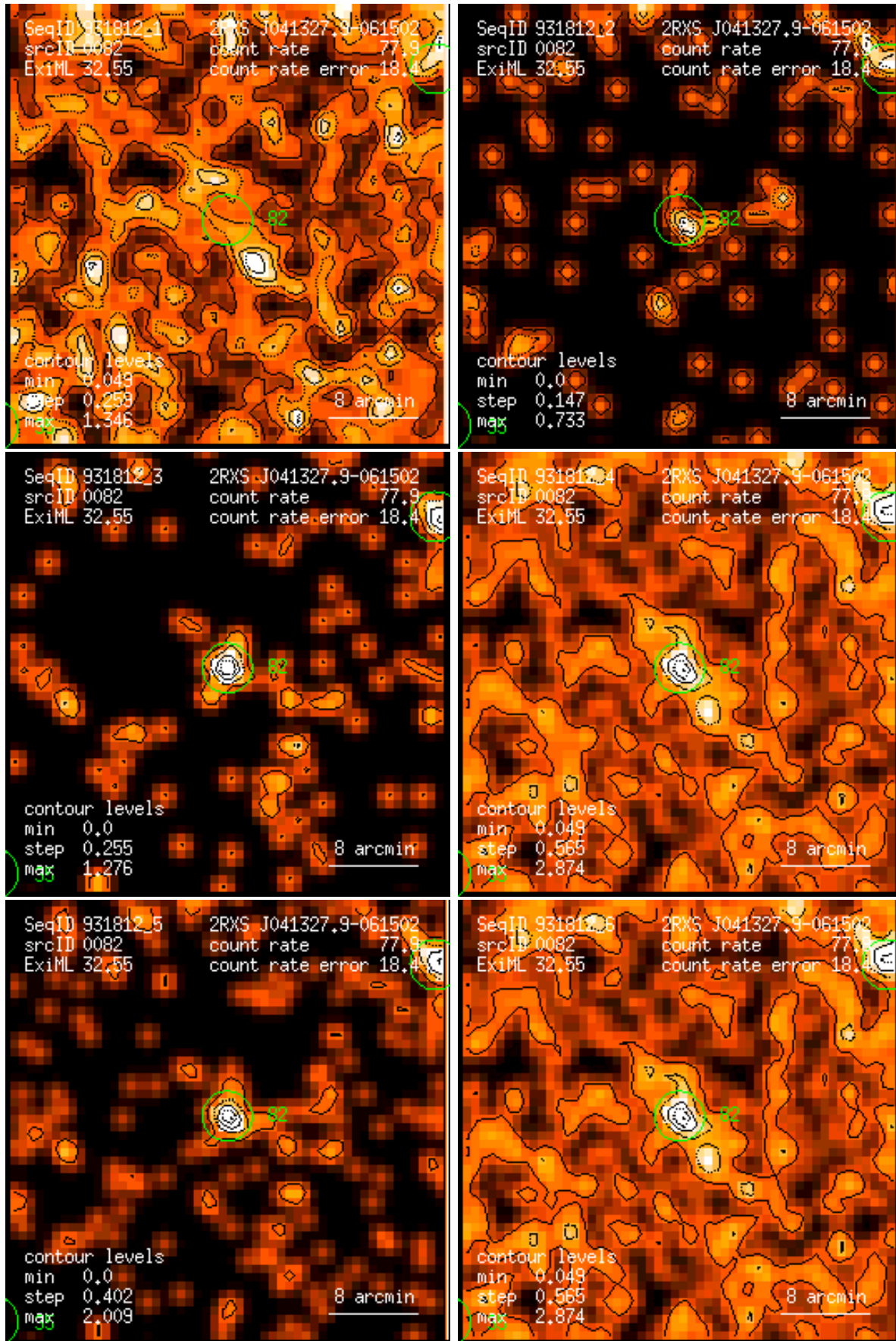
Figure 82: RASS 931812: detection 0082: band rate images, Gaussian filter: (1) PSPC channels 11 – 41, (2) 52 – 90, (3) 91 – 201, (4) 11 – 235, (5) 52 – 201, (6) 11 – 201. Broad band rates in counts/ks. Band rate contour levels in counts/ks/arcmin 2 .
