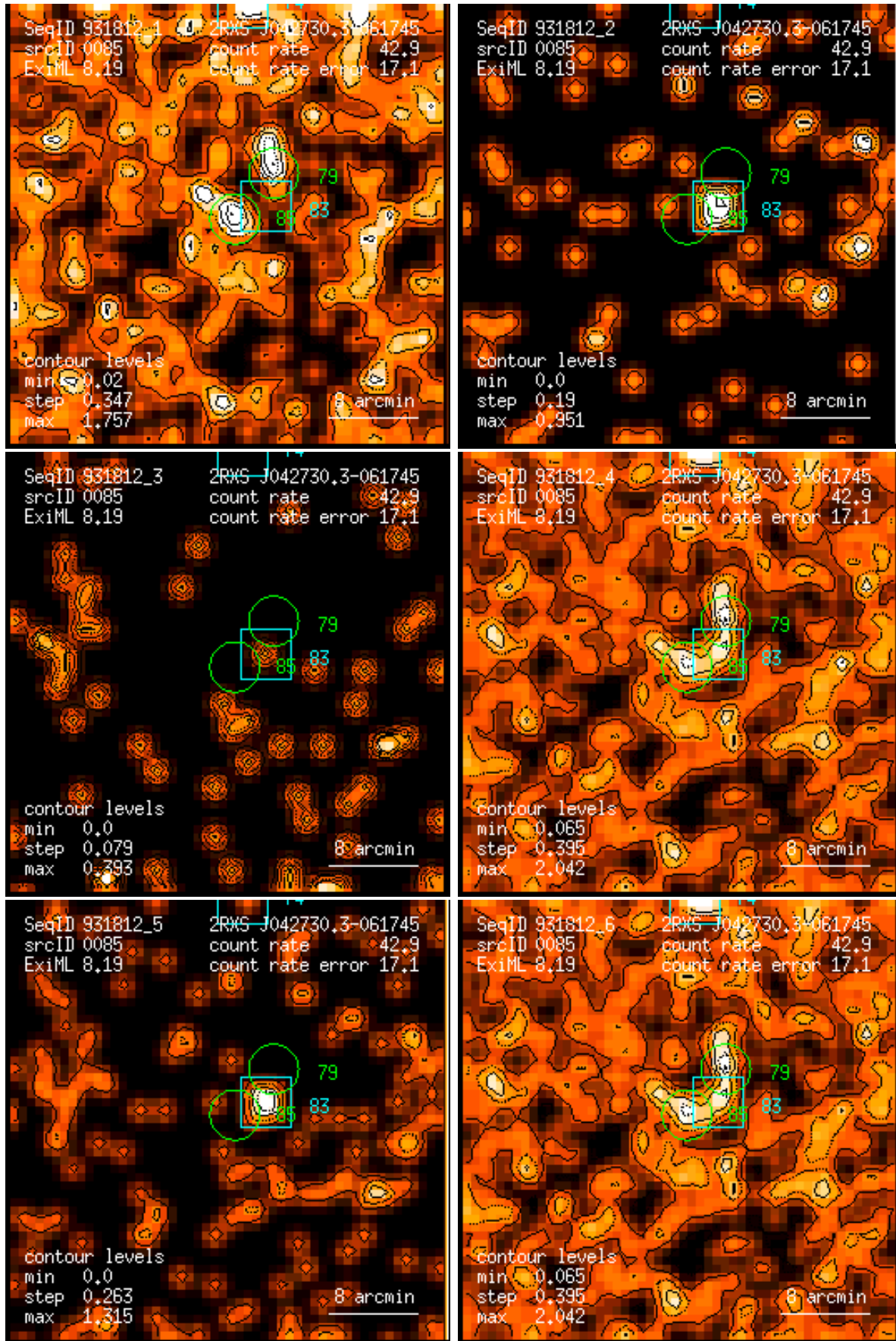
Figure 85: RASS 931812: detection 0085: band rate images, Gaussian filter: (1) PSPC channels 11 – 41, (2) 52 – 90, (3) 91 – 201, (4) 11 – 235, (5) 52 – 201, (6) 11 – 201. Broad band rates in counts/ks. Band rate contour levels in counts/ks/arcmin 2 .
