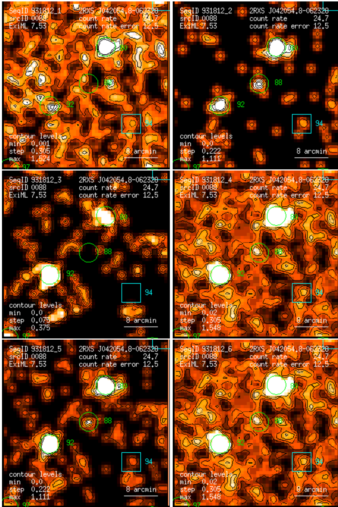
Figure 88: RASS 931812: detection 0088: band rate images, Gaussian filter: (1) PSPC channels 11 – 41, (2) 52 – 90, (3) 91 – 201, (4) 11 – 235, (5) 52 – 201, (6) 11 – 201. Broad band rates in counts/ks. Band rate contour levels in counts/ks/arcmin 2 .
