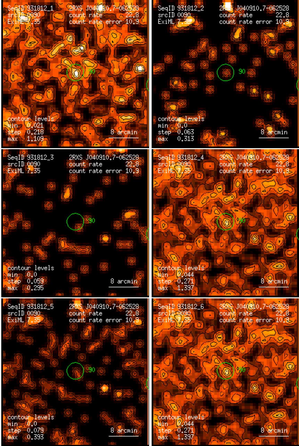
Figure 90: RASS 931812: detection 0090: band rate images, Gaussian filter: (1) PSPC channels 11 – 41, (2) 52 – 90, (3) 91 – 201, (4) 11 – 235, (5) 52 – 201, (6) 11 – 201. Broad band rates in counts/ks. Band rate contour levels in counts/ks/arcmin 2 .
