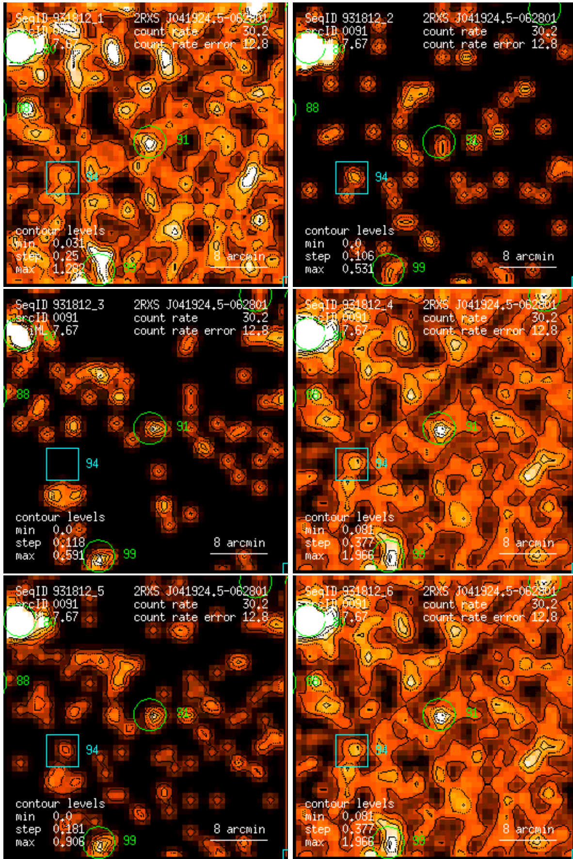
Figure 91: RASS 931812: detection 0091: band rate images, Gaussian filter: (1) PSPC channels 11 – 41, (2) 52 – 90, (3) 91 – 201, (4) 11 – 235, (5) 52 – 201, (6) 11 – 201. Broad band rates in counts/ks. Band rate contour levels in counts/ks/arcmin 2 .
