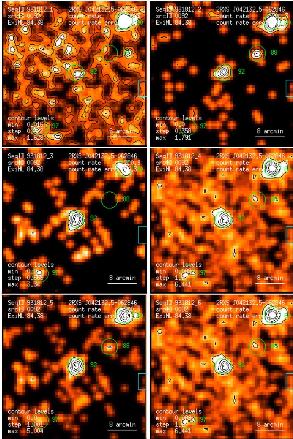
Figure 92: RASS 931812: detection 0092: band rate images, Gaussian filter: (1) PSPC channels 11 – 41, (2) 52 – 90, (3) 91 – 201, (4) 11 – 235, (5) 52 – 201, (6) 11 – 201. Broad band rates in counts/ks. Band rate contour levels in counts/ks/arcmin 2 .
