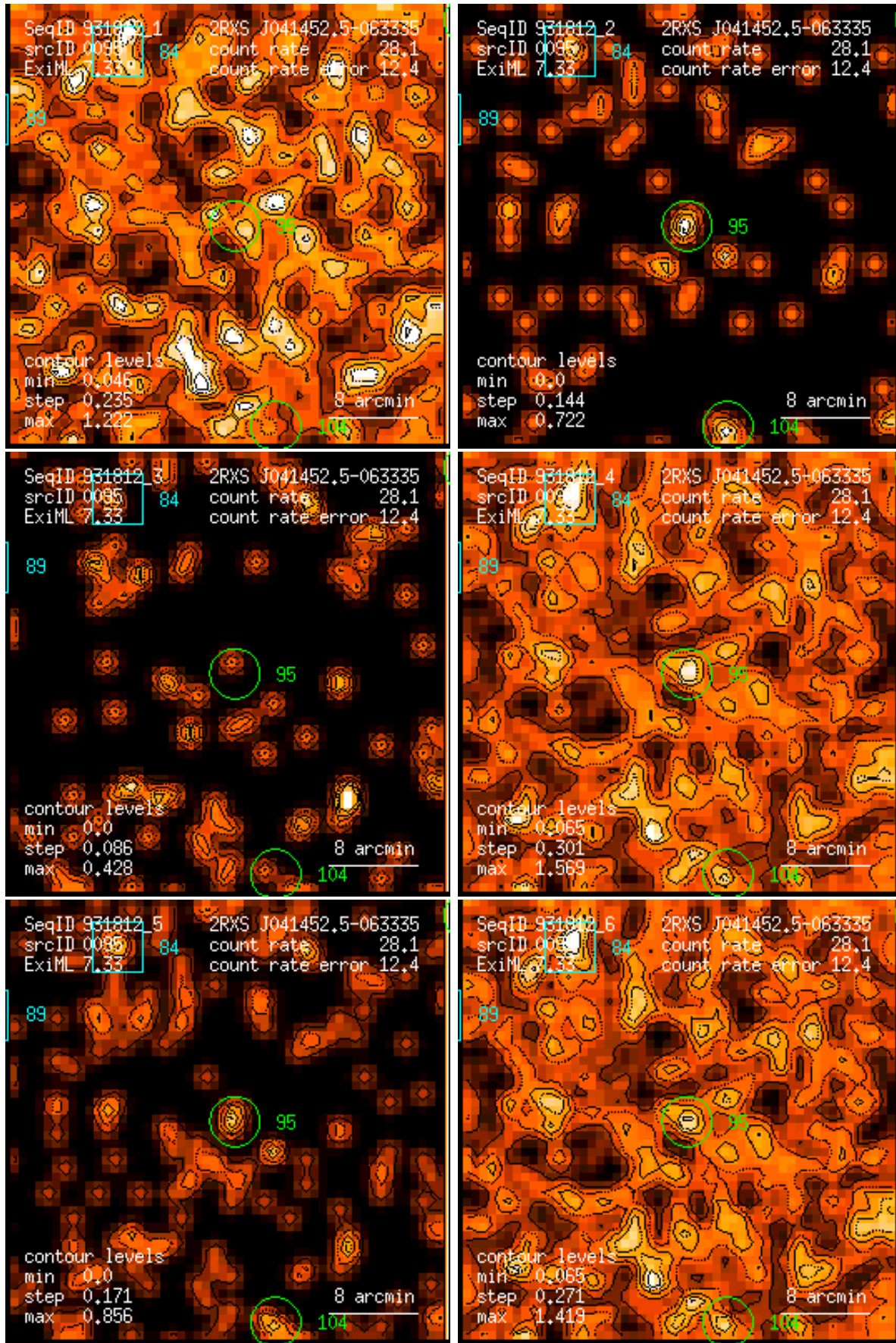
Figure 95: RASS 931812: detection 0095: band rate images, Gaussian filter: (1) PSPC channels 11 – 41, (2) 52 – 90, (3) 91 – 201, (4) 11 – 235, (5) 52 – 201, (6) 11 – 201. Broad band rates in counts/ks. Band rate contour levels in counts/ks/arcmin 2 .
