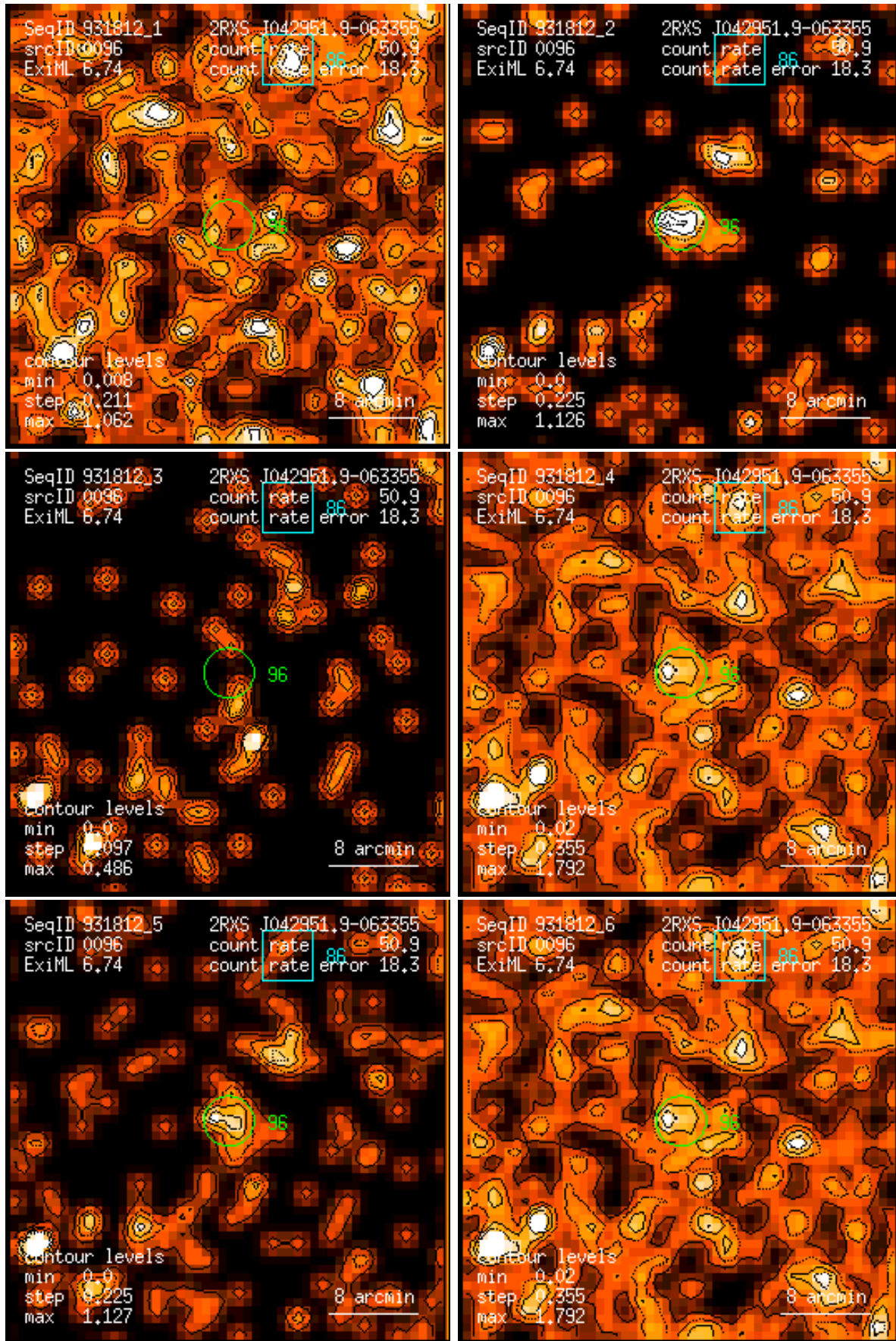
Figure 96: RASS 931812: detection 0096: band rate images, Gaussian filter: (1) PSPC channels 11 – 41, (2) 52 – 90, (3) 91 – 201, (4) 11 – 235, (5) 52 – 201, (6) 11 – 201. Broad band rates in counts/ks. Band rate contour levels in counts/ks/arcmin 2 .
