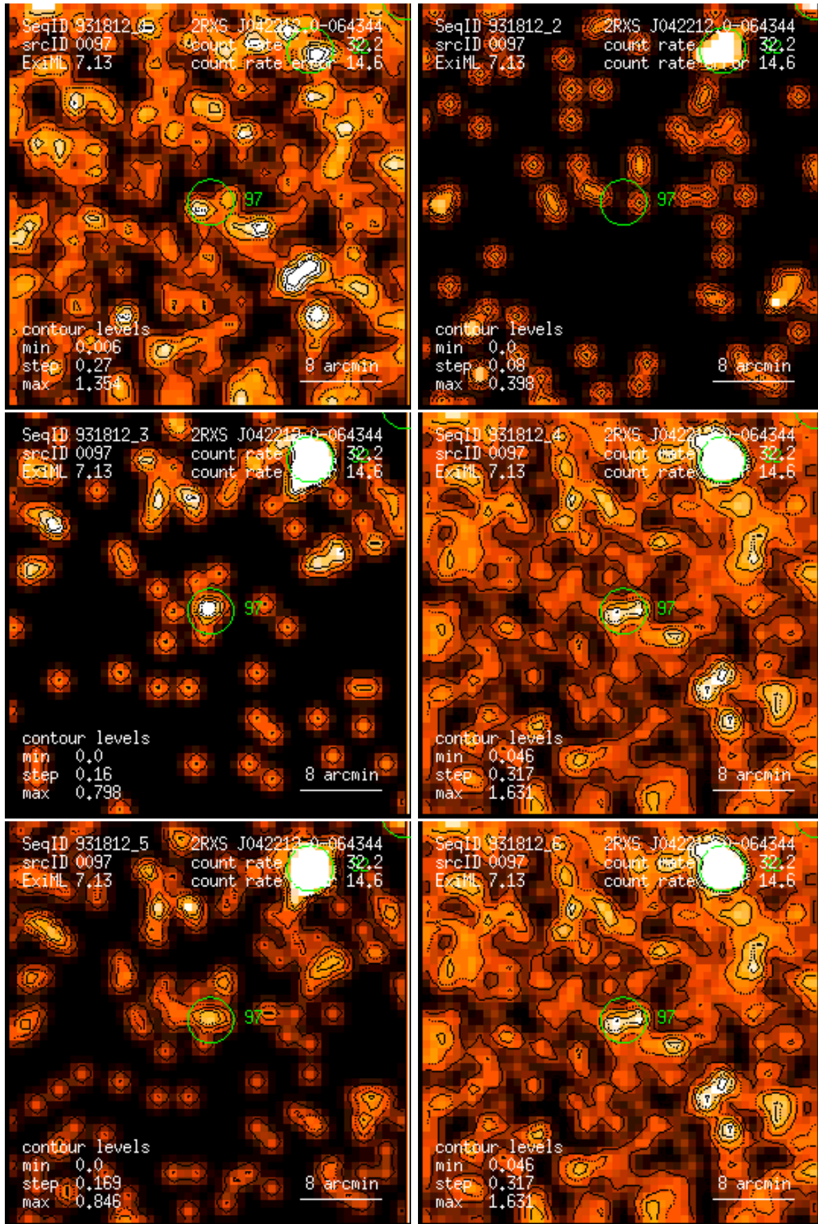
Figure 97: RASS 931812: detection 0097: band rate images, Gaussian filter: (1) PSPC channels 11 – 41, (2) 52 – 90, (3) 91 – 201, (4) 11 – 235, (5) 52 – 201, (6) 11 – 201. Broad band rates in counts/ks. Band rate contour levels in counts/ks/arcmin 2 .
