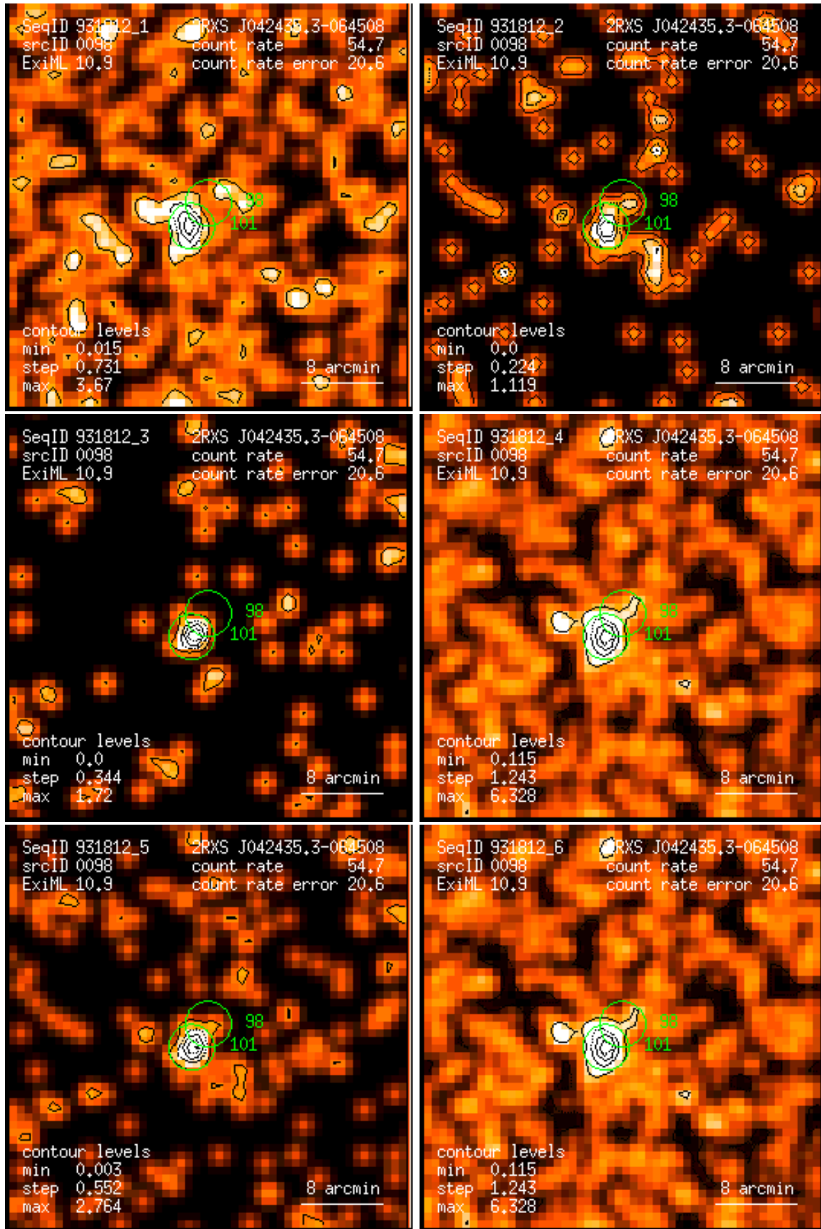
Figure 98: RASS 931812: detection 0098: band rate images, Gaussian filter: (1) PSPC channels 11 – 41, (2) 52 – 90, (3) 91 – 201, (4) 11 – 235, (5) 52 – 201, (6) 11 – 201. Broad band rates in counts/ks. Band rate contour levels in counts/ks/arcmin 2 .
