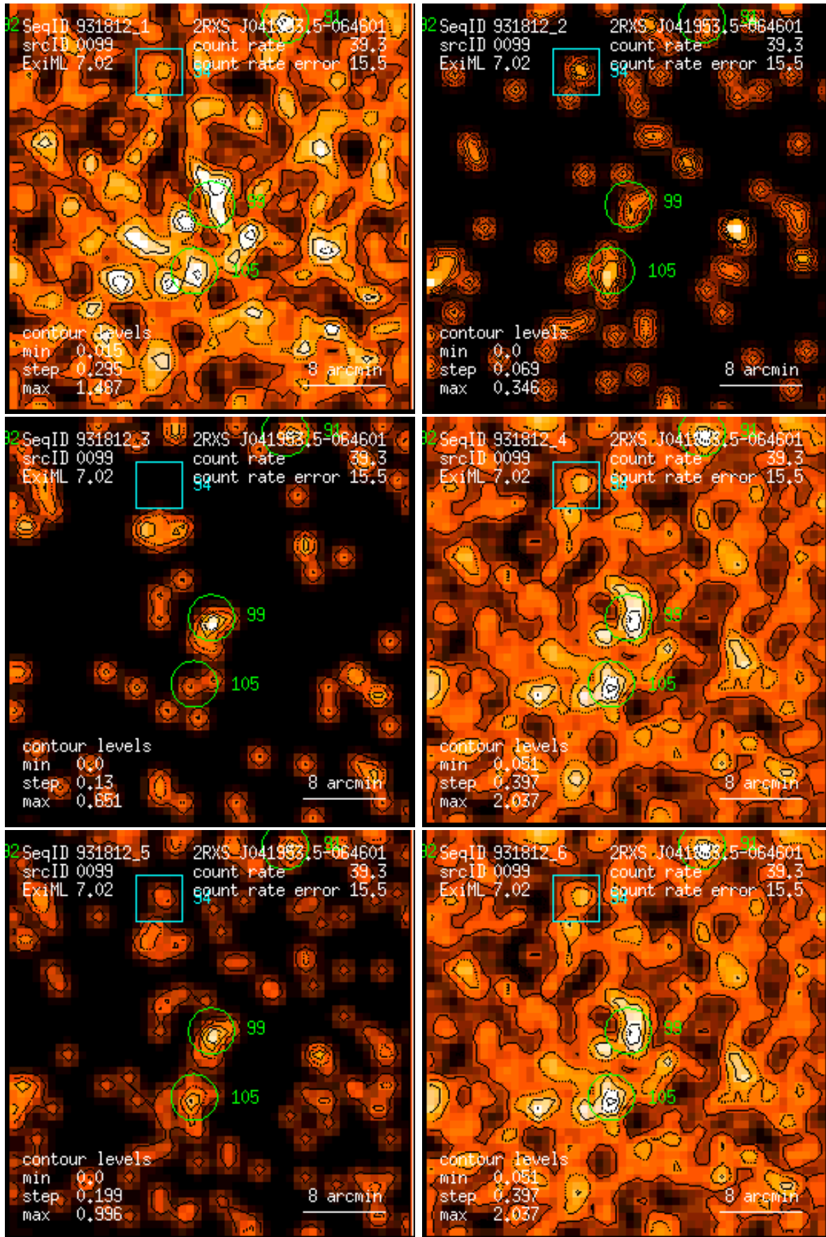
Figure 99: RASS 931812: detection 0099: band rate images, Gaussian filter: (1) PSPC channels 11 – 41, (2) 52 – 90, (3) 91 – 201, (4) 11 – 235, (5) 52 – 201, (6) 11 – 201. Broad band rates in counts/ks. Band rate contour levels in counts/ks/arcmin 2 .
