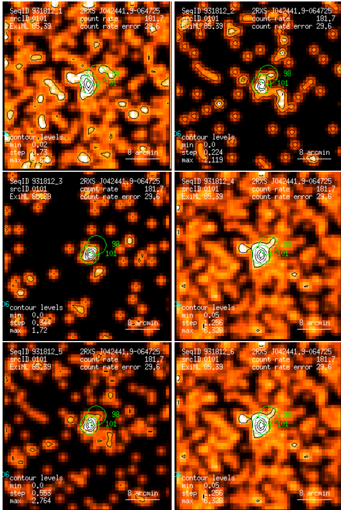
Figure 101: RASS 931812: detection 0101: band rate images, Gaussian filter: (1) PSPC channels 11 – 41, (2) 52 – 90, (3) 91 – 201, (4) 11 – 235, (5) 52 – 201, (6) 11 – 201. Broad band rates in counts/ks. Band rate contour levels in counts/ks/arcmin 2 .
